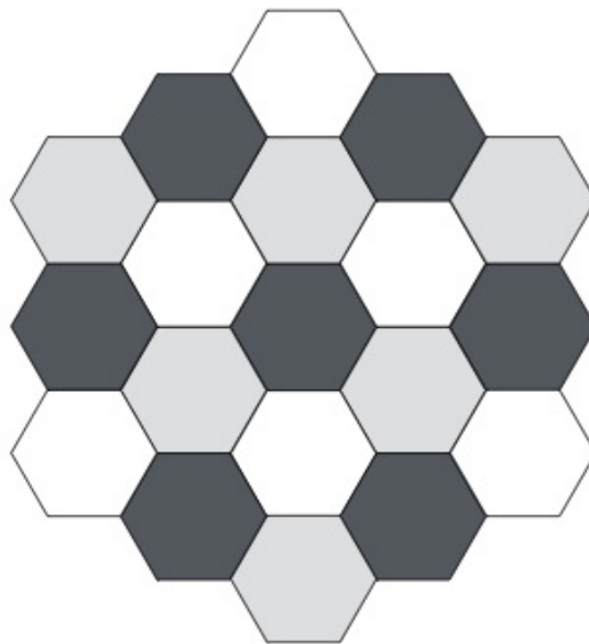
FIGURE 10. Belov's 3-colored pattern of the tiling of the plane by regular hexagons (Senechal, 1988). The tiling pattern is said to be 'perfect' as every operation in G is associated with a unique colour permutation (Senechal, 1988).
