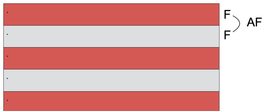
FIGURE 4. Landau modelled the layered structures of various transition metal halides as strongly interacting layers (ferromagnetically coupled) that were negatively coupled by a much weaker energy (Landau, 1933).
