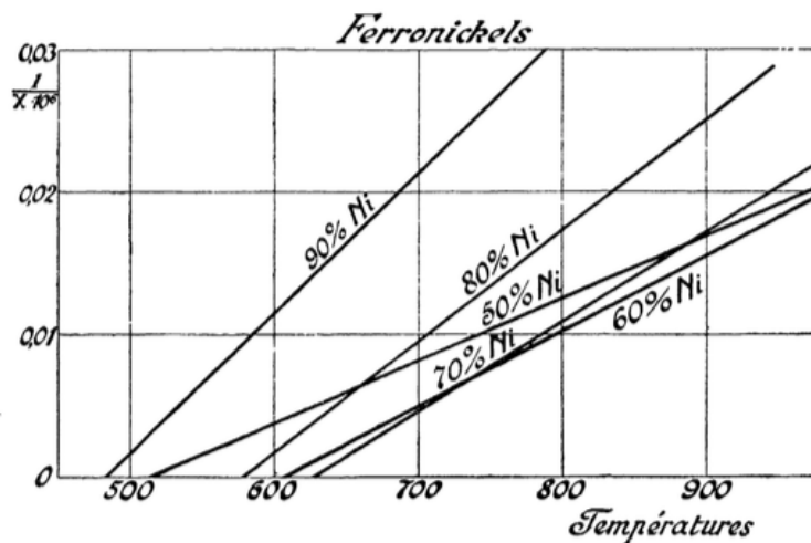
FIGURE 2. The commonly observed linear decrease in the inverse susceptibility upon cooling became known as the Curie law . This dependence is exemplified by data taken from a variety of iron/nickel alloys (Weiss and Foex, 1911).
