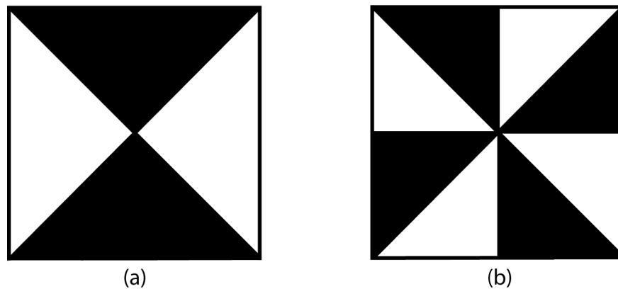
FIGURE 8. Black and white squares to illustrate the black and white point groups (a) 4'mm' and (b) 4m'm' (Cracknell, 1969).
