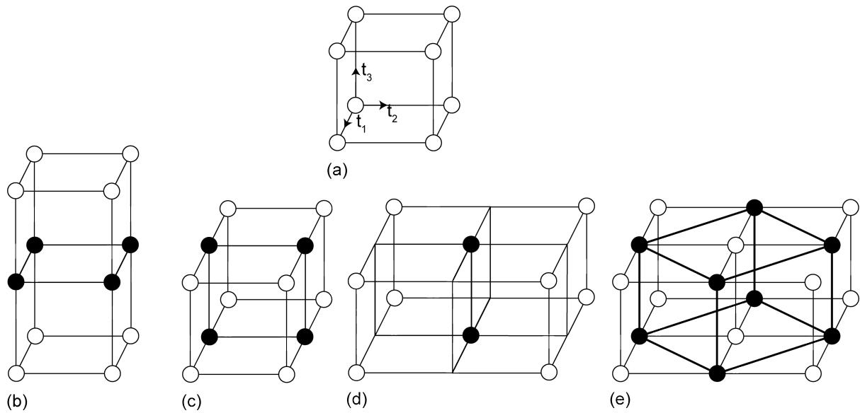
FIGURE 9. The black and white lattices, or dichromatic Bravais lattices, created from a tetragonal unit cell (a) (Izyumov, 1980).
