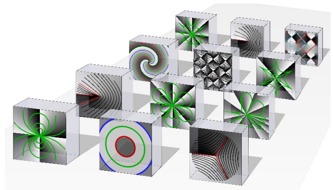
Figure 2: Overview of 12 different polarization singular structures visualized by corresponding Stokes field phase (back) and sketches of flow and singular lines and points (front).
