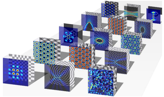
Figure 1: Overview of 15 exemplary, structured light fields with corresponding amplitude (front) and phase (back) distributions, respectively.
