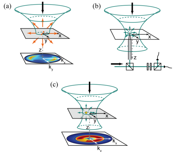
Figure 2 – Selected schemes for the measurement of highly confined polarization distributions. (a) Direct mapping of individual field components using single fluorescence molecules. (b) Coherent measurement of field components by NSOM. (c) Full field reconstruction with a single scattering nanoprobe and angularly resolved far-field detection of the transmission signal.
