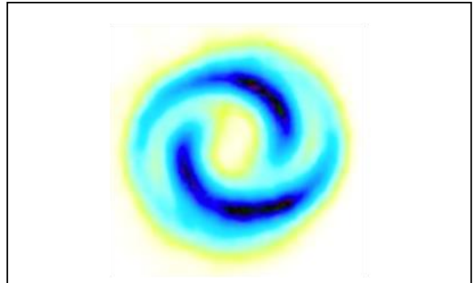
Figure 1 – The density profile of one spin state of a spinor BEC that has counterrotating azimuthal phase twists (counter rotating vortices) and a radial phase gradient. See ref [6].
