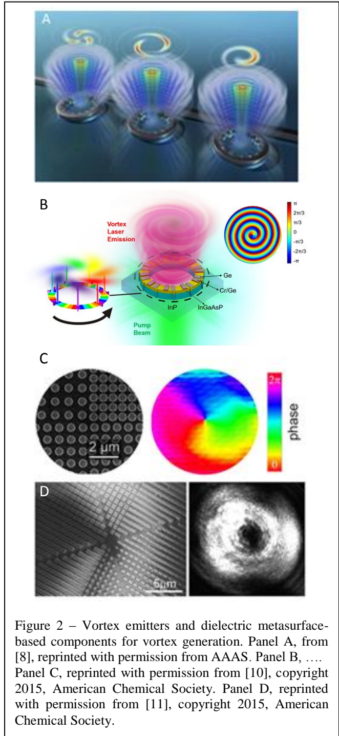
Figure 2 – Vortex emitters and dielectric metasurface-based components for vortex generation. Panel A, from [8], reprinted with permission from AAAS. Panel B, ... Panel C, reprinted with permission from [10], copyright 2015, American Chemical Society. Panel D, reprinted with permission from [11], copyright 2015, American Chemical Society.
