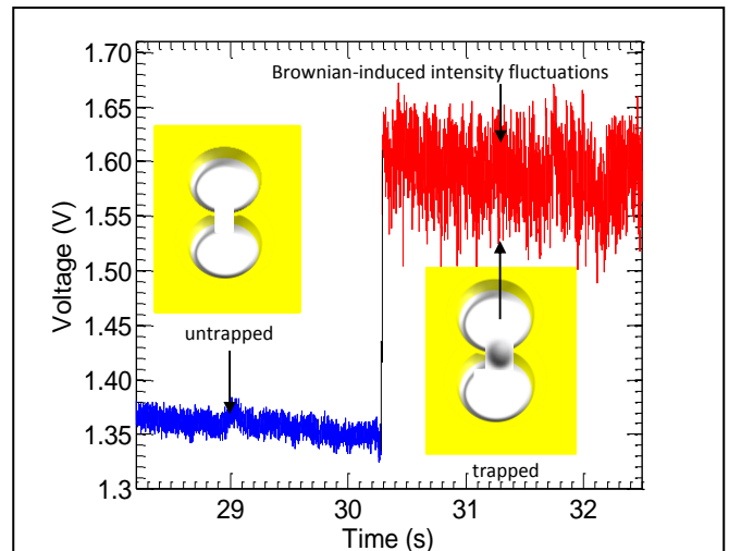
Figure 1 – Change in laser transmission through a double nanohole in 100 nm thick gold film with trapping of 20 nm diameter polystyrene sphere (nanoparticle) in solution. The transmission is proportional to the avalanche photodetector voltage. An abrupt step occurs at trapping (20% jump in transmission), as well as an increase in intensity fluctuations from Brownian motion of the nanoparticle.
