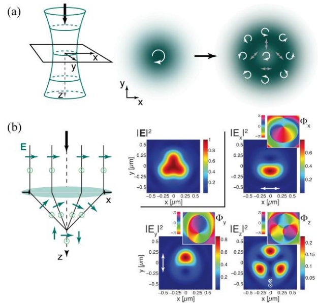
Figure 1 – (a) In paraxial light fields, the lateral polarization structure can be transformed from homogeneous to inhomogeneous distributions. (b) Sketch of tight focusing of polarized light beams (left), resulting in complex focal field distributions (right, from [5]. Reprinted with permission from AAAS).
