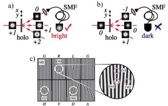
Fig. 2. Scheme for quantum state tomography of qutrits using holograms. The target mode couples to the detector (a), while any other mode is rejected (b). The 8-segment analysis hologram need not measure all 3-mode superpositions, it is enough to measure 2-part superpositions. {G, R, L, H, V, D, A} correspond to the main spatial mode analyzed by that segment. The positions (i)–(iii) and (iv)–(vi) correspond to degenerate and non-degenerate qubits respectively. (Reprinted with permission from [9], Copyright (2004) by the American Physical Society.)
