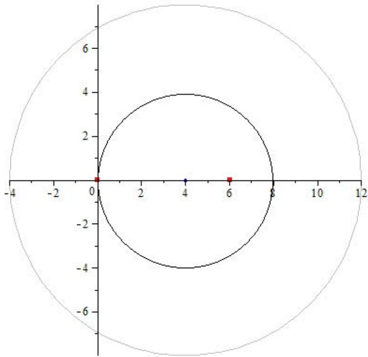
FIGURE 1. The Gershgorin disk and half-disk of H
