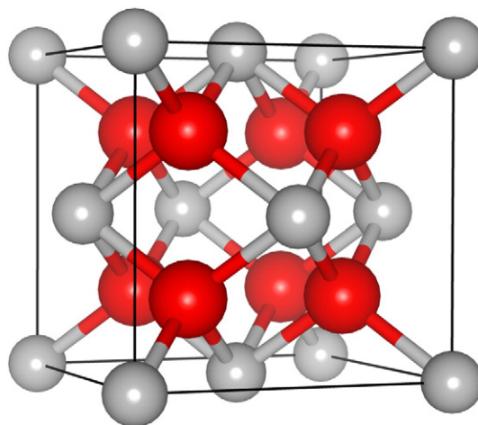
Fig. 1. Crystal structure of cubic zirconia (c- \text{ZrO}_2 ). Colour key: oxygen and zirconium atoms are represented by red and grey spheres, respectively.
