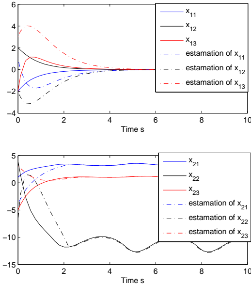
Fig. 1. The time response of both 1st and 2nd subsystems, the states x_1 = \text{col}(x_{11}, x_{12}, x_{13}) and their estimation \hat{x}_1 = \text{col}(\hat{x}_{11}, \hat{x}_{12}, \hat{x}_{13}) , the states x_2 = \text{col}(x_{21}, x_{22}, x_{23}) and their estimation \hat{x}_2 = \text{col}(\hat{x}_{21}, \hat{x}_{22}, \hat{x}_{23})
