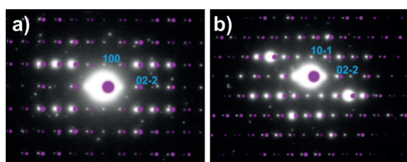
Figure 5. Comparison of the experimental TEM electron diffraction patterns of flsZ with patterns simulated from the PXRD-derived crystal structure of flsZ . The patterns were indexed to the \langle 011 \rangle (a) and \langle 111 \rangle (b) zone axes of this structure. Simulated patterns are shown in purple and offset slightly relative to the experimental electron diffraction patterns for clarity. The simulated diffraction patterns were modeled assuming the kinematic model of electron scattering. The effects of dynamic scattering in the experimental patterns lead to appearance of reflections that are absent under the kinematic model. [32]
