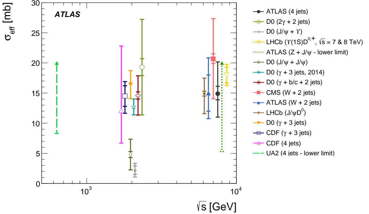
Figure 9: The effective overlap area between the interacting hadrons, \sigma_{\text{eff}} , as a function of the centre-of-mass energy, \sqrt{s} , for different processes and in different experiments [17–30]. The inner error bars (where visible) correspond to the statistical uncertainties and the outer error bars represent the sum in quadrature of the statistical and systematic uncertainties. Dashed arrows indicate lower limits. For clarity, measurements at identical centre-of-mass energies are slightly offset in \sqrt{s} .
