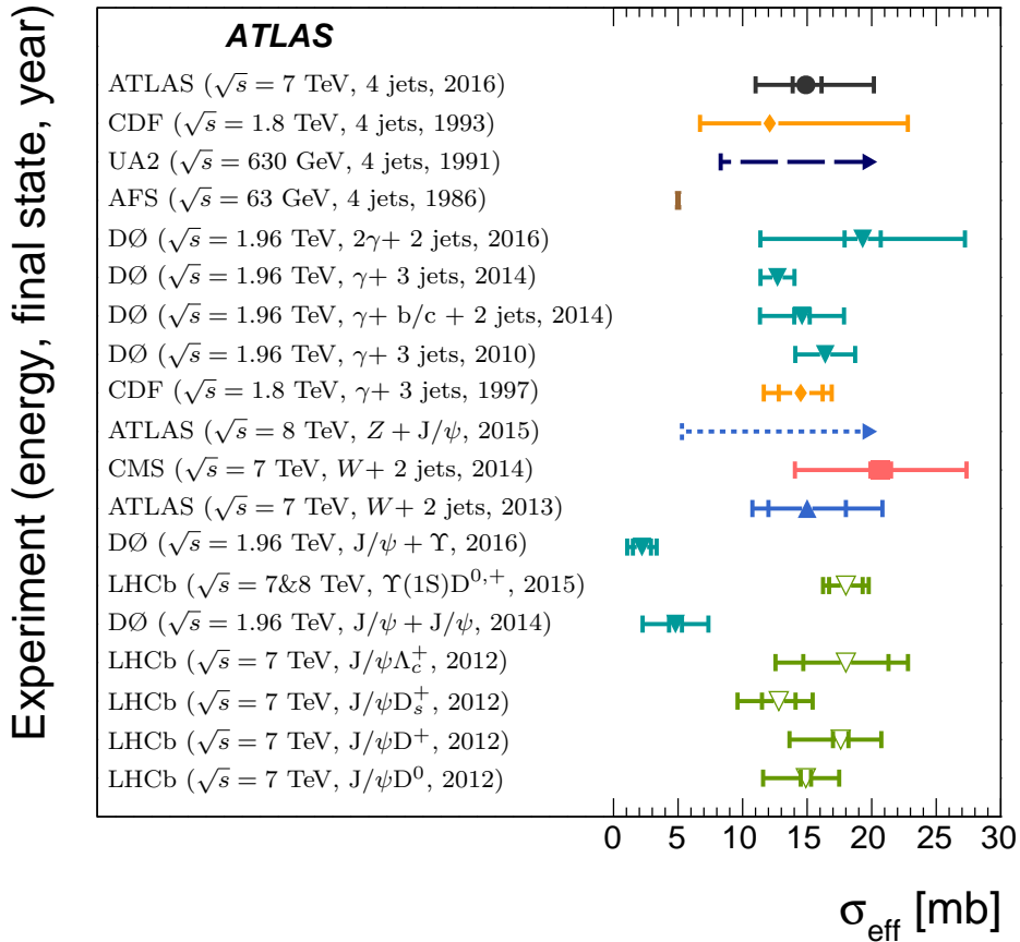
Figure 8: The effective overlap area between the interacting hadrons, \sigma_{\text{eff}} , determined in various final states and in different experiments [16–30]. The inner error bars (where visible) correspond to the statistical uncertainties and the outer error bars represent the sum in quadrature of the statistical and systematic uncertainties. Dashed arrows indicate lower limits and the vertical line represents the AFS measurement published without uncertainties.
