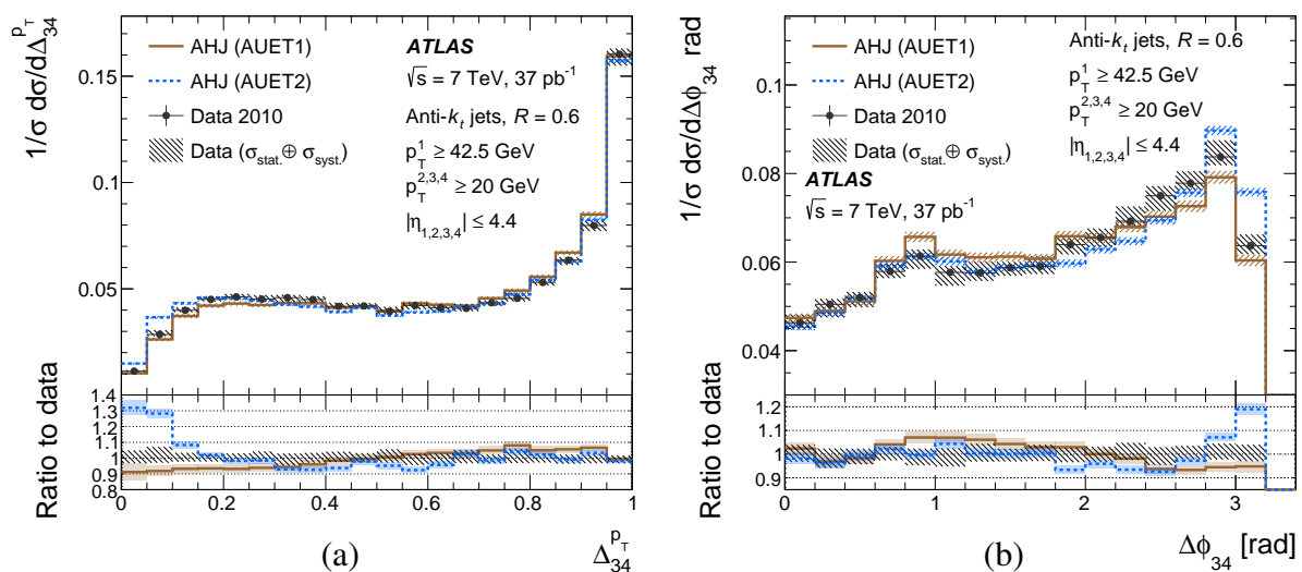
Figure 10: Distributions of the variables (a) \Delta_{34}^{p_T} and (b) \Delta\phi_{34} , defined in Eq. (16), in data after unfolding to particle level, compared to the MC prediction from AHJ at the particle level, generated using the AUET1 and AUET2 tunes, as indicated in the legend. The hatched area represents the sum in quadrature of the statistical and systematic uncertainties in the normalized differential cross-sections and all histograms are normalized to unity. The ratio of the particle-level distribution to the normalized differential cross-section is shown in the bottom panels, where the shaded areas represent statistical uncertainties.
