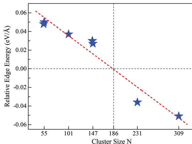
Fig. 7 REE as a function of nanocluster size N . The REEs are obtained by the fitting method as shown in Fig. 5(a) for Ru_{54} and Ru_{55} , Fig. 6 for Ru_{146} , Ru_{147} , and Ru_{309} , Fig. S4† for Ru_{101} and Fig. S5† for Ru_{231} , respectively.
