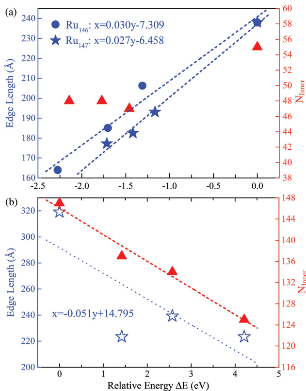
Fig. 6 The least squares fitting of the relative energies as a function of the total edge length of (a) three FCCCF and the I_h cluster for both Ru_{146} and Ru_{147} cluster series; (b) three FCCCF configurations and the I_h - Ru_{309} clusters. For both Ru_{147} and Ru_{309} , the numbers of inner atoms in clusters ( N_{inner} ) represented by the triangles (in red) versus relative energy are also shown. The geometry configurations of Ru_{147} and Ru_{309} are shown in Fig. 3(II) and (III), respectively.
