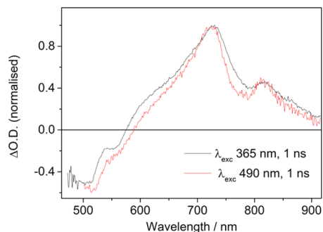
Figure 3. TA spectrum of PBI-A in water (pH 9) at 47 mM showing the presence of the same transient species 1 ns after excitation following initial excitation of either the S_0 – S_2 (365 nm) or S_0 – S_1 (490 nm) transitions.
