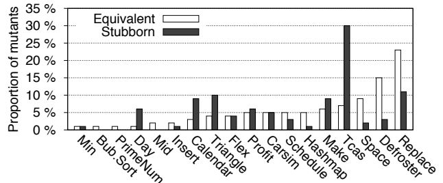
Figure 2: The proportionate contribution of the mutants from each program to the total number of all equivalent and all stubborn mutants (as a percentage of all mutants)
