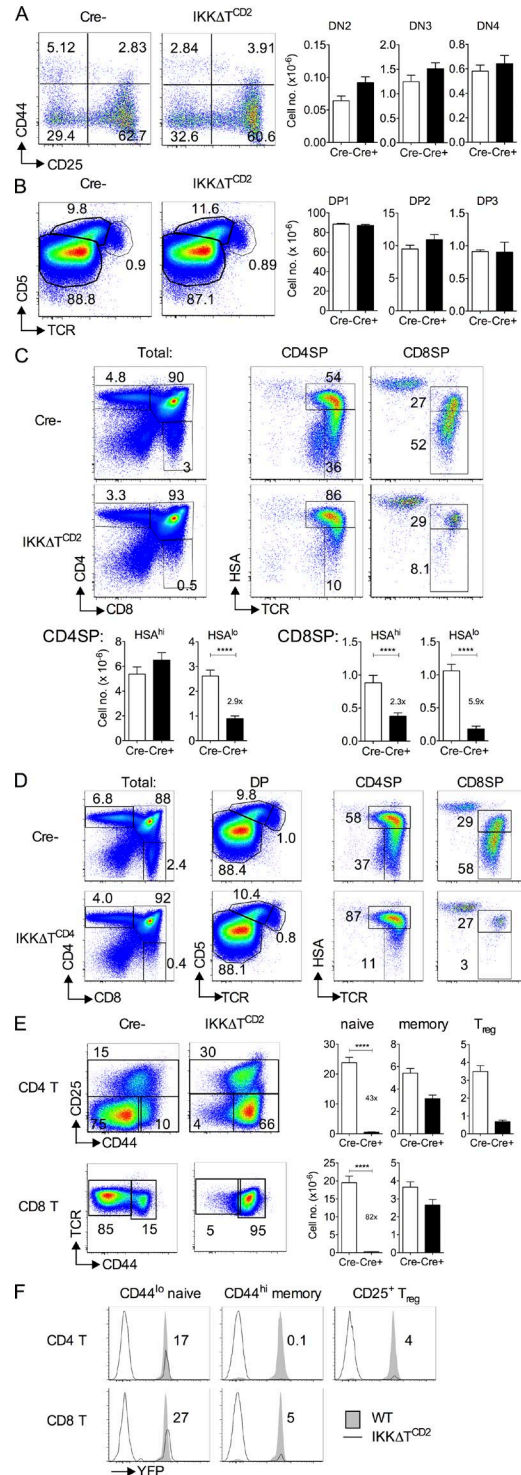
Figure 1. Deletion of Ikk1 and Ikk2 blocks SP thymocyte development. Lymphoid organs from 8–12-wk-old Ikk1 flx/flx Ikk2 flx/flx Rosa26 R YFP huCD2 iCre (IKK \Delta T CD2 , n = 16 ) were analyzed by FACS and compared with huCD2 iCre -ve (Cre - , n = 15 ) littermate as control. (A) Density plots are of CD44 versus CD25 by DN Lin - (CD4, CD8, TCR \alpha , and CD5) thymocytes. Numbers indicate percentage in the corresponding quadrant. Bar charts are cell number of CD44 hi CD25 hi (DN2), CD44 lo CD25 hi (DN3), and CD44 lo
