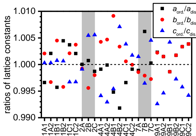
Fig. 8 Ratios of the lattice constants obtained from DFT calculations of the various homo -network structures with respect to the lattice constants of a fully hydrogen-disordered 3 \times 3 \times 3 supercell. The first number of the labels of the structures is the number of the space group and followed by the type of networks the structure contains. For some combinations there are two distinct structures for a given space group and network type.
