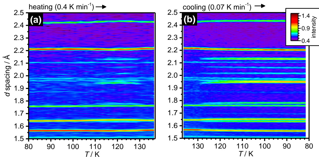
Fig. 2 Powder neutron diffraction data of pressure-quenched 0.01 mol L -1 DCl-doped ice VI recorded (a) upon heating at 0.4 K min -1 and (b) subsequent cooling at 0.07 K min -1 at ambient pressure. Diffraction intensity at ~2.1 Å is due to vanadium from the sample container.
