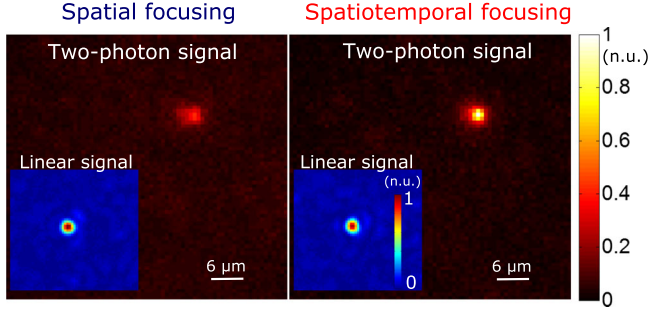
FIG. 3. Comparison of two-photon excitation for spatial (monochromatic phase conjugation) and spatiotemporal focusing, obtained with a thinner scattering sample of ZnO ( \tau_m \approx 500 fs). Inset: corresponding CCD signal. Integration time identical for both excitations: 2s for the two-photon excitation and 1 ms for the linear excitation. Scale bars normalized to the maximum intensity of spatiotemporal focusing. We observe a twofold enhancement of the nonlinear signal for the same average intensity when performing spatiotemporal focusing.
