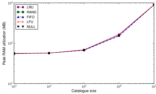
Figure 4: Peak RAM utilization vs. content catalogue size
