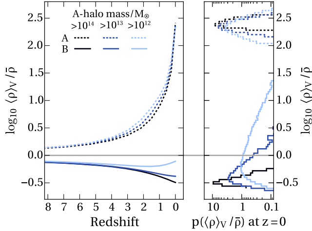
FIG. 2. The volume-averaged density of Lagrangian regions corresponding to z = 0 A-halos of different mass ranges (from darkest to lightest: 10^{14} < M/M_{\odot} < 10^{15} , 10^{13} < M/M_{\odot} < 10^{14} and 10^{12} < M/M_{\odot} < 10^{13} respectively). The left panel shows the evolution of each mass bin’s mean density; the right panel shows the spread of halo-averaged densities within the bin at z = 0 . Dashed lines show the regions in the A simulation (so at z = 0 these correspond to halos); solid lines show the corresponding “antihalo” regions in the B simulation. The most massive antihalos can be identified as voids. At lower masses there is a tail of crushed, high-density antihalos, reflecting the known void-in-cloud evolution asymmetry.
