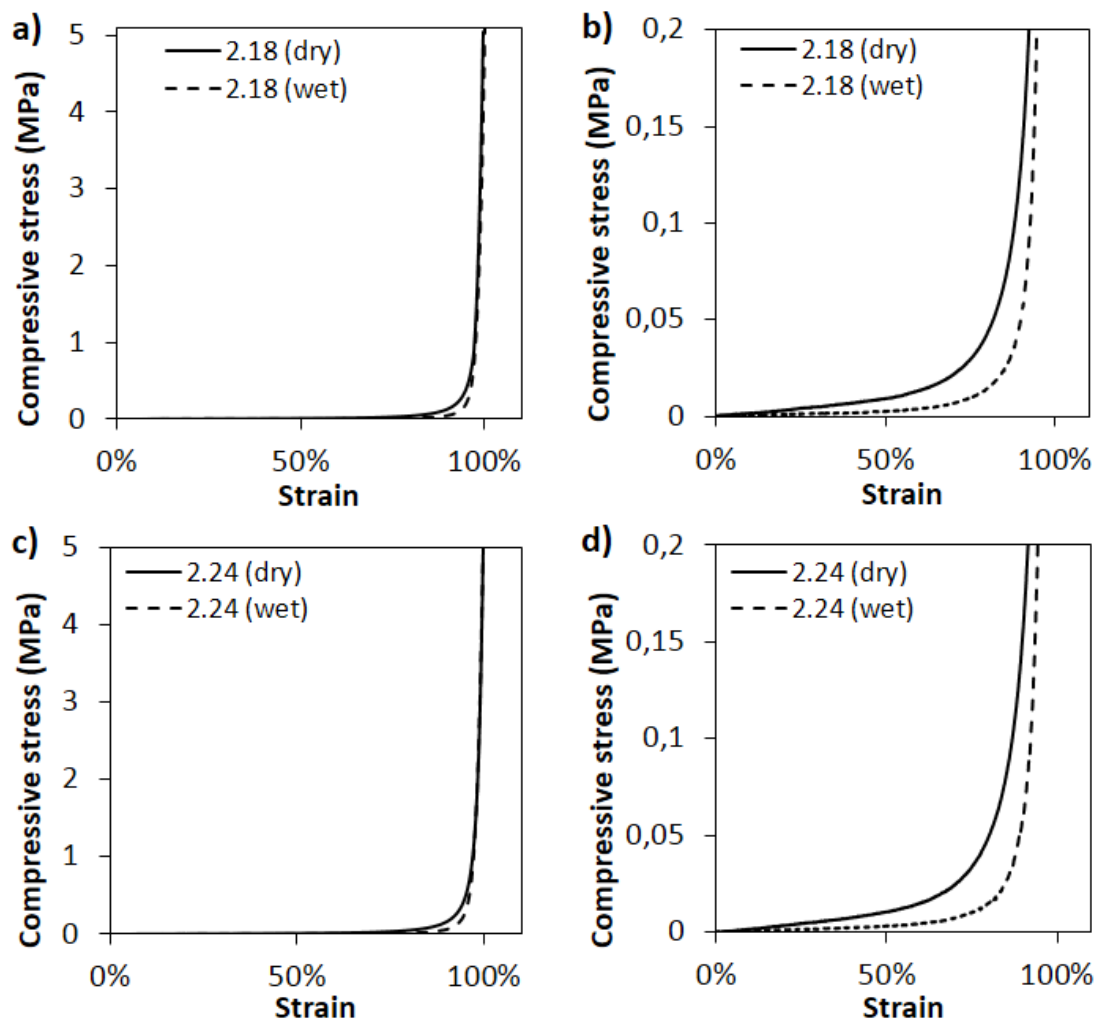
Figure S4. Compressive stress-strain curves of the GO-Col scaffolds at pH 2. a-b) 18% of collagen/GO w/w ratio; c-d) 24% of collagen / GO w/w ratio.
