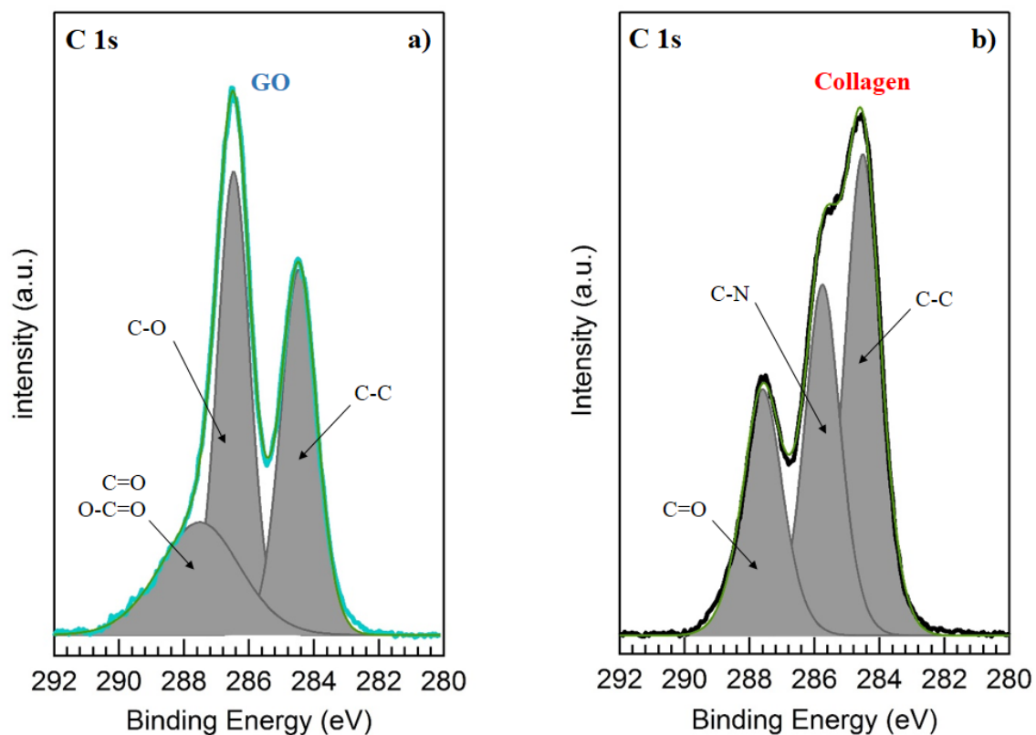
Figure S2. Normalized C1s core levels obtained for a) GO and b) collagen.
