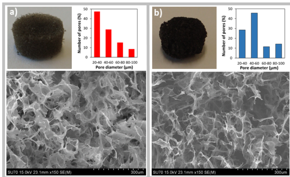
Figure 4. Microporous architecture of a) the GO-Col and b) rGO-Col scaffolds, showing in both cases a photograph of the scaffold, the correspondent SEM microstructure and the pore size distribution.
