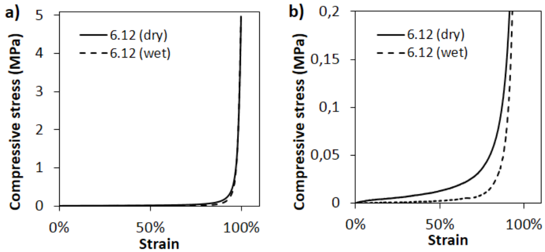
Figure S6. Compressive stress-strain curves of the GO-Col scaffolds at pH 6. a-b) 18% of collagen/GO w/w ratio.
