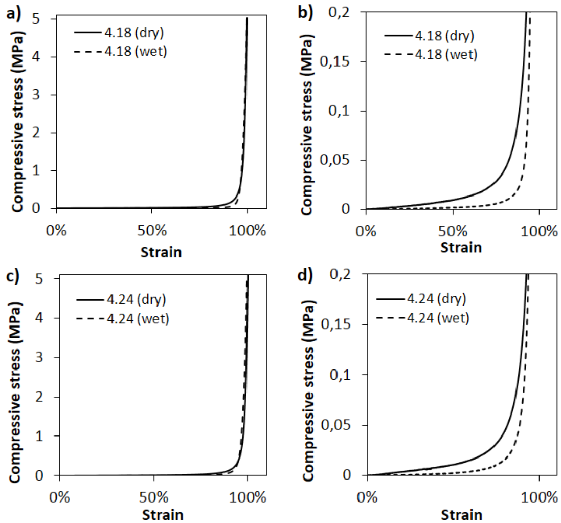
Figure S5. Compressive stress-strain curves of the GO-Col scaffolds at pH 4. a-b) 18% of collagen/GO w/w ratio; c-d) 24% of collagen / GO w/w ratio.
