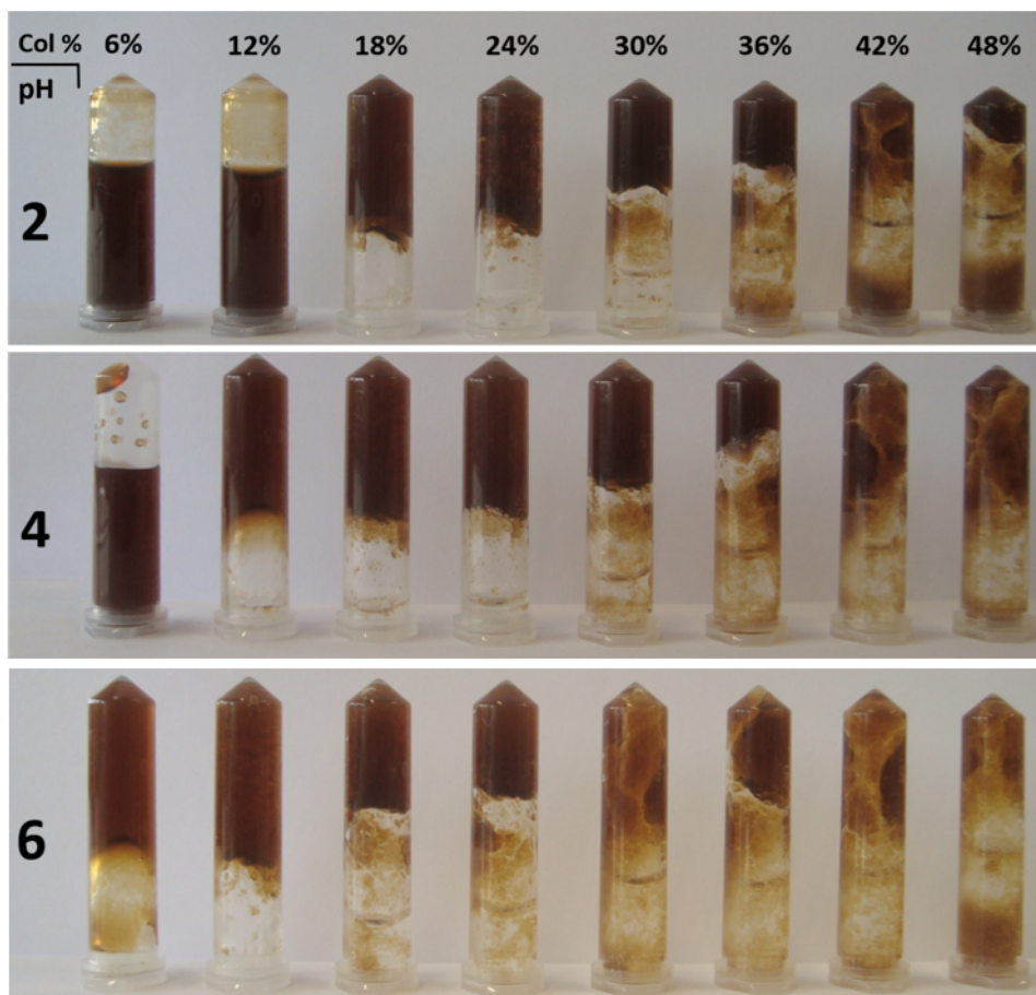
Figure S1. Photographs of 4 mg/mL GO solutions mixed and shaken with collagen at different weight ratios and pH values: 2; 4 and 6. From left to right, Col/GO (w/w %) = 6, 12, 18, 24, 30, 36, 42 and 48.
