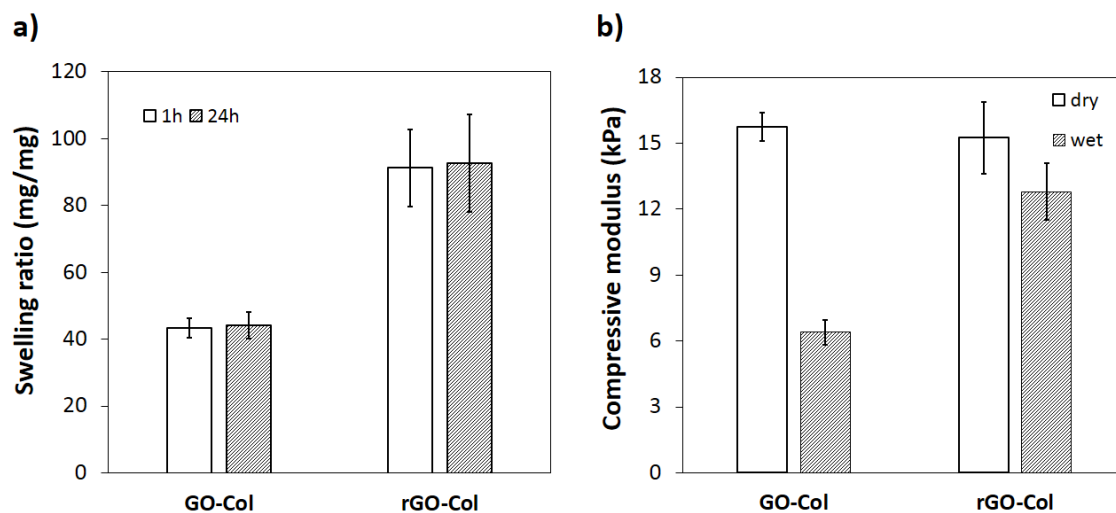
Figure S 8. Comparison of a) the swelling ratio and b) compressive modulus of the GO-Col and rGO-Col.
