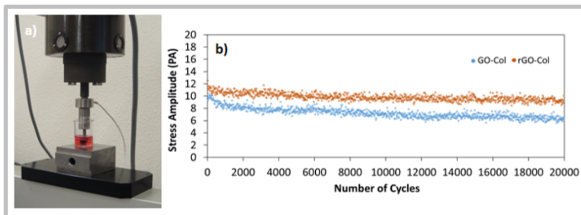
Figure 6. Comparison of the mechanical response of the GO-Col and rGO-Col scaffolds under dynamic compression cycles. a) Dynamic compression system apparatus; b) Stress amplitude versus number of cycles curves of the GO-Col scaffold (blue) and its reduced counterpart (orange).
