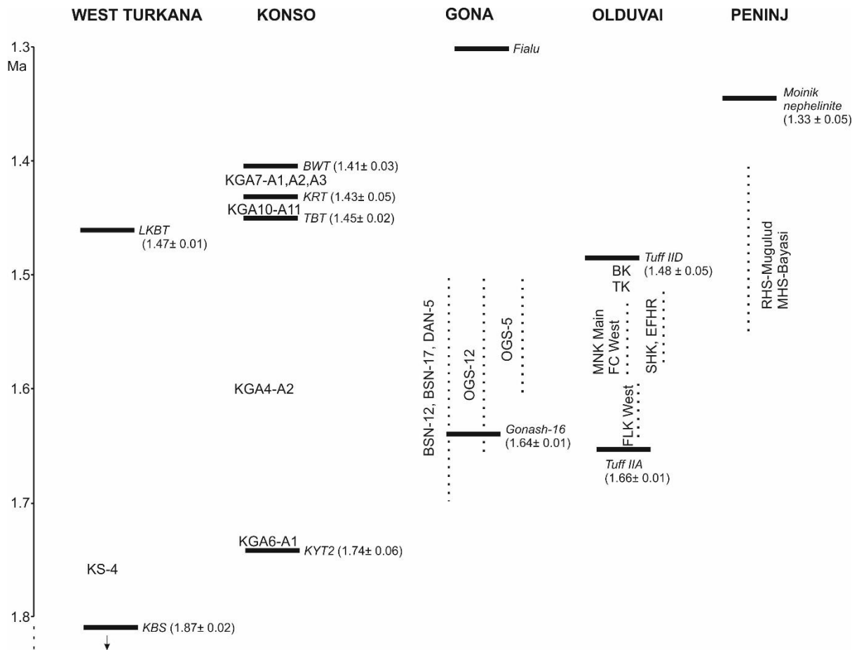
Figure 2. Chronostratigraphy* of selected** early handaxe-bearing assemblages in East Africa. West Turkana ages from [57]. Konso: [74]. Gona: [58,75]. Olduvai***: [66]. Peninj: [45]. *Only sites with an estimated age of >1.2 Myr are included. **Both Melka Kunture and Gadeb may contain Early Acheulean assemblages around 1.4 Ma ago (see reviews by [3,61]), but minimum ages are < 1Myr [62,64], and therefore these sites are not included in the figure. *** Manega [66]'s dating is here selected over other radiometric results for Tuff IIA [42] and Tuff IID [65], and a regionally uncorrelated tuff (FLKWb) dated at 1.698 Ma [67]. Bars and names in italics refer to local tuffs.
