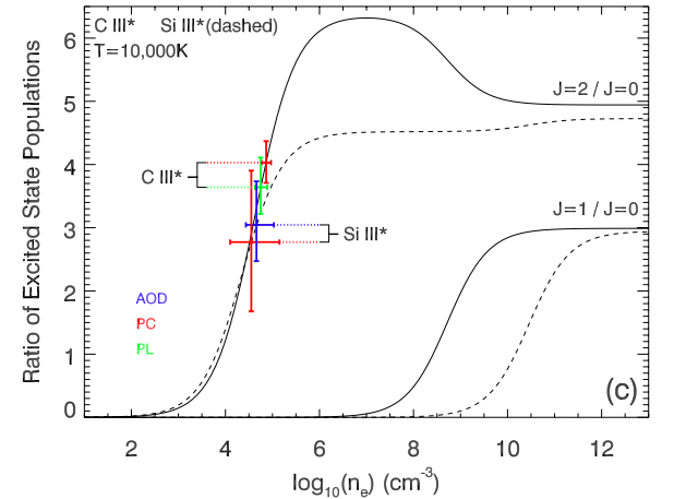
Fig. 4. a) Absorption spectrum for the C III* 1175 Å multiplet. The 2013 COS spectrum shows clear and relatively unblended individual troughs from the J = 2 and J = 0 levels, but no contribution from the J = 1 level that is populated at higher densities (see panel c). b) Absorption spectrum for the Si III* 1298 Å multiplet (similar in level structure to the C III* 1175 Å multiplet). The 2013 COS spectrum shows shallow but highly significant individual troughs from the J = 2 and J = 0 levels, but again no contribution from the J = 1 level that is populated at higher densities. c) C III* and Si III* level population ratios, theory and measurements. The computed populations for the J = 2/J = 0 and J = 1/J = 0 are plotted as a function of electron number density for both ions (see text for elaboration). The crosses show the measured ratios for the J = 2/J = 0 ratio of both ions. From the C III* ratios we infer \log(n_e) = 4.8 \pm 0.1 \text{ cm}^{-3} , where the error includes both statistical and systematic effects. This value is fully consistent with the one inferred from the Si III* ratio, where in the case of Si III* the statistical error is larger since the troughs are much shallower.
