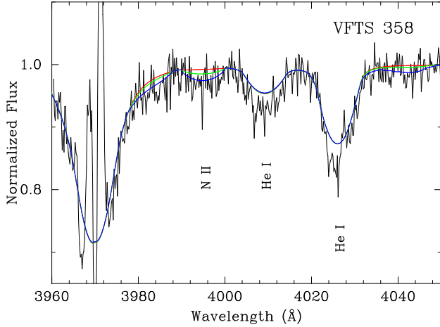
Fig. 8. Section of the VFTS 358 spectrum showing, from left-to-right, the He I, N II \lambda 3995 , and He I \lambda 4009 , 4026 lines; we note that He I is complicated by absorption from the interstellar Ca H line (as well as nebular emission). Model spectra for our adopted physical parameters and 12 + \log(\text{N}/\text{H}) = 6.9, 7.7, and 8.5 , are overplotted in red, green, and blue, respectively.
