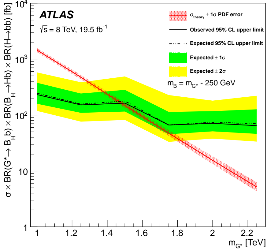
Figure 4: Observed (solid) and expected (dashed) 95% C.L. upper limits on the cross section \sigma(pp \rightarrow G^* \rightarrow B_H \bar{b}) \times \text{BR}(B_H \rightarrow Hb) \times \text{BR}(H \rightarrow b\bar{b}) for VLQ mass points with m_{B_H} = m_{G^*} - 250 GeV, from the combined merged and resolved analyses, as well as the theoretical prediction based on parameters given in Section 3. The uncertainty band around the theory cross section reflects the uncertainty in the CTEQ6.6 PDFs.
