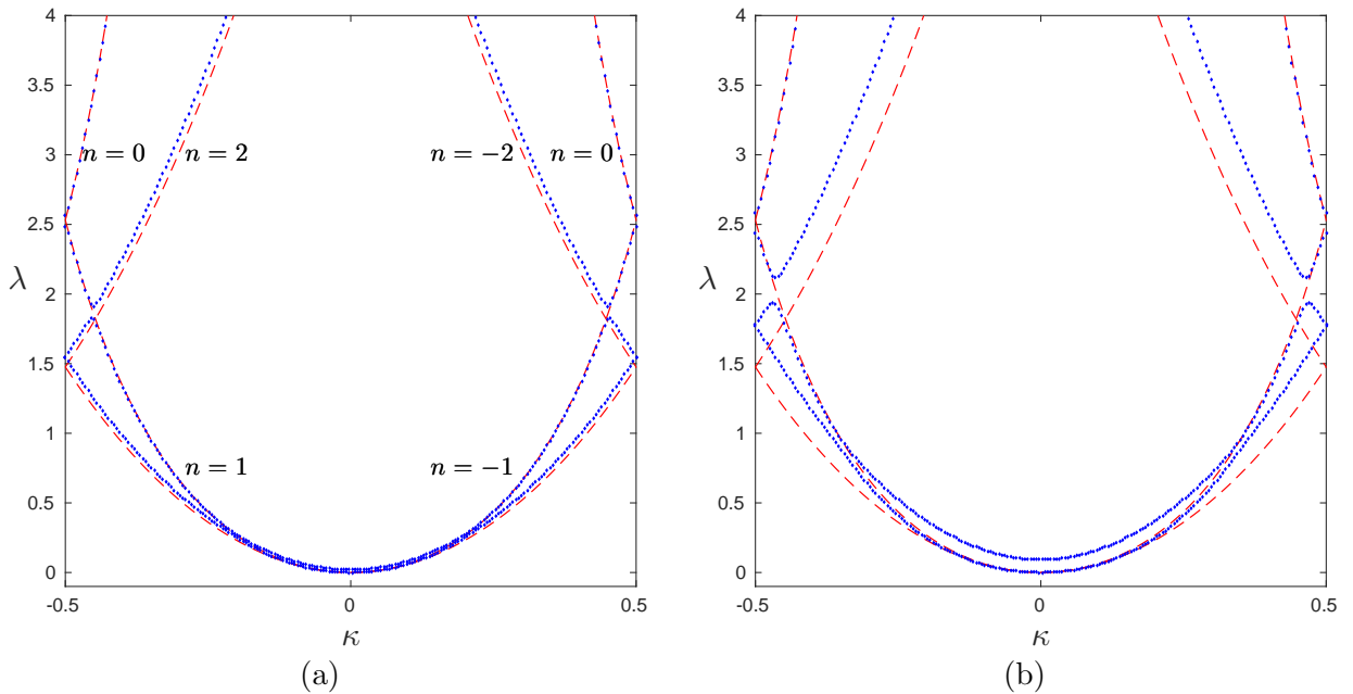
Figure 2: The lowest eigenvalues of the operator (5.5) as a function of \kappa when c = 0.5 for (a) a = -0.1 and (b) a = -0.2 . The dashed lines (red online) give the lowest eigenvalues of the unperturbed operator for a = 0 and the computed eigenvalues are shown as diamonds (blue online). All repeated eigenvalues for a = 0 are split as a \neq 0 .
