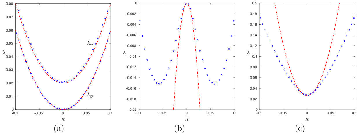
Figure 3: (a) A detail of figure 2(a) (for c = 0.5 and a = -0.1 ) in the neighbourhood of the origin showing the splitting of the two spectral bands at finite a . (b) The ground spectral band for a = -0.1 but for c = 0.7 . (c) The first excited spectral band for a = -0.1 and c = 0.7 . The dashed lines here give the small- \kappa , small- a asymptotic expansions (4.9) and (4.10) for the two spectral bands.
