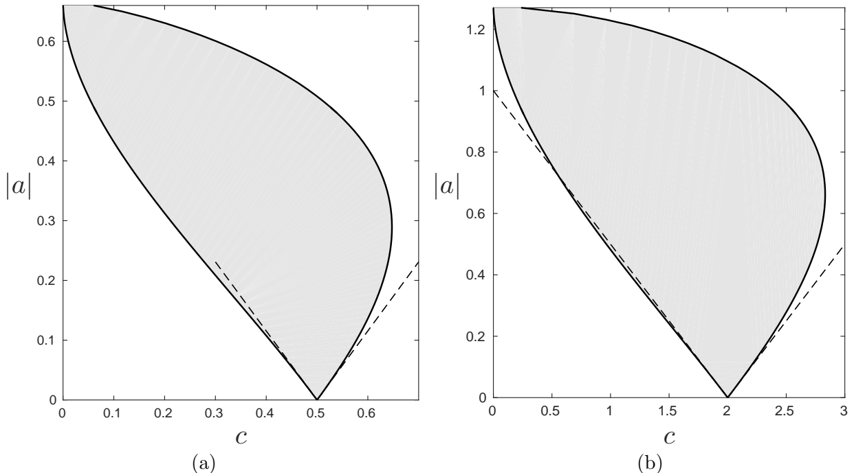
Figure 4: The region of the (c, |a|) plane where the operator P_{c,\gamma}(\kappa) is positive for all \kappa is shown shaded for the reduced Ostrovsky equation (a) and the reduced modified Ostrovsky equation (b). The dashed lines show the asymptotic expansions for the boundary for small |a| as given by (2.42) and (3.25) respectively.
