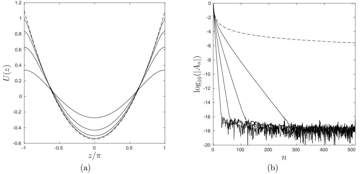
Figure 1: (a) The 2\pi -periodic solutions of the reduced Ostrovsky equation (2.2) for a = -0.3, -0.5, -0.6, -0.65 . (b) The logarithm of the absolute value of the Fourier cosine coefficients, A_n , of the trigonometric approximation (5.2). The limiting piecewise parabolic wave, corresponding to a = -\frac{2}{3} is shown dashed in (a) with the corresponding coefficients A_n = 2(-1)^n/3n^2 included in (b).
