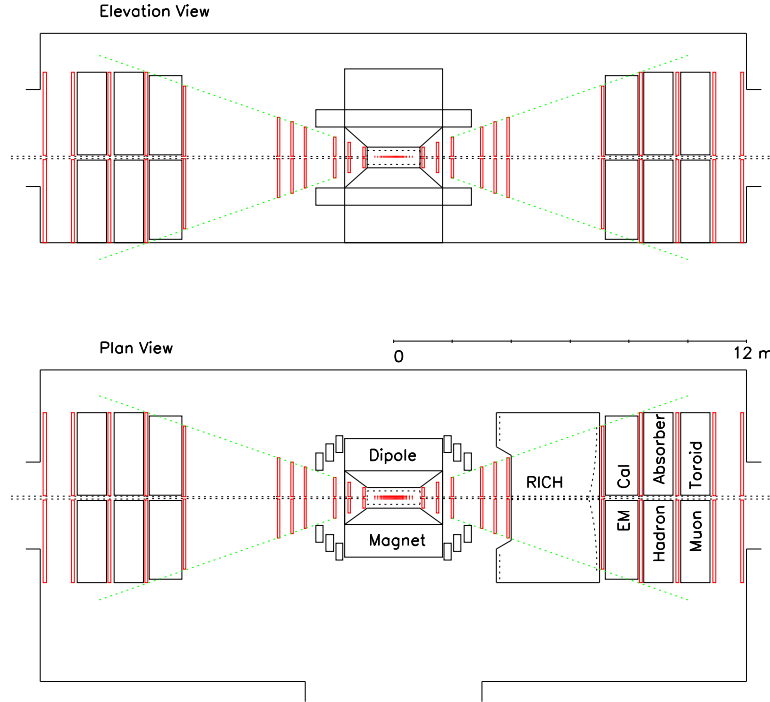
Figure 11: Schematic Layout of the BTeV detector
