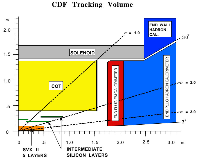
Figure 8: Longitudinal View of the CDF II Tracking System.
