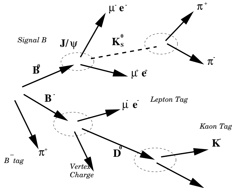
Figure 4: Example of B tagging.
