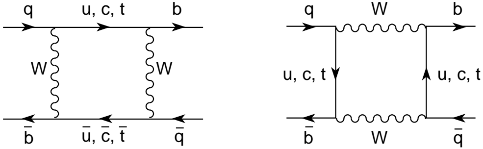
Figure 2: B^0 - \bar{B}^0 mixing diagrams.
