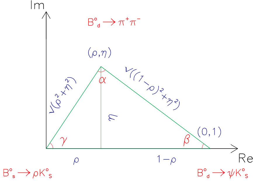
CKM triangle
