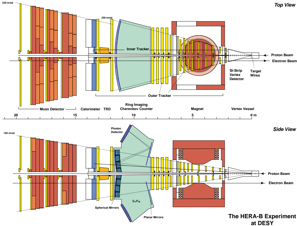
Figure 6: Schematic of the HERA-B detector at DESY.
