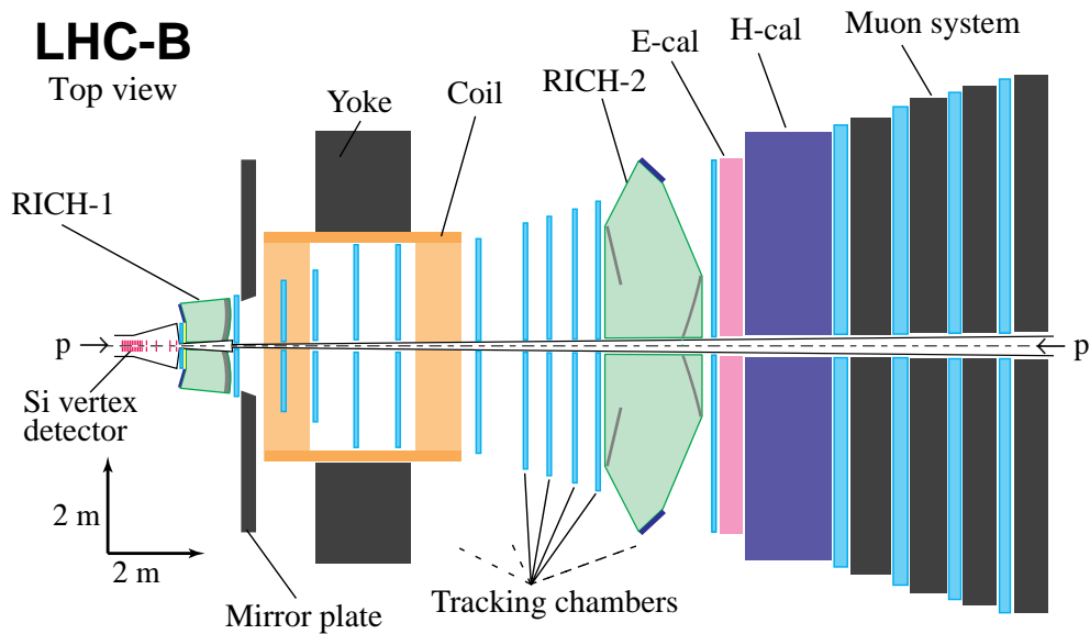
Figure 10: Top view of the LHC-B detector
