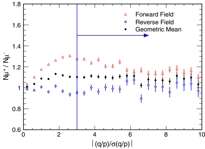
FIG. 1. Charge ratio for reconstructed multiple-muon tracks as a function of curvature significance after applying all other selection cuts. The vertical line denotes the minimum value for tracks used in the charge ratio measurement.
