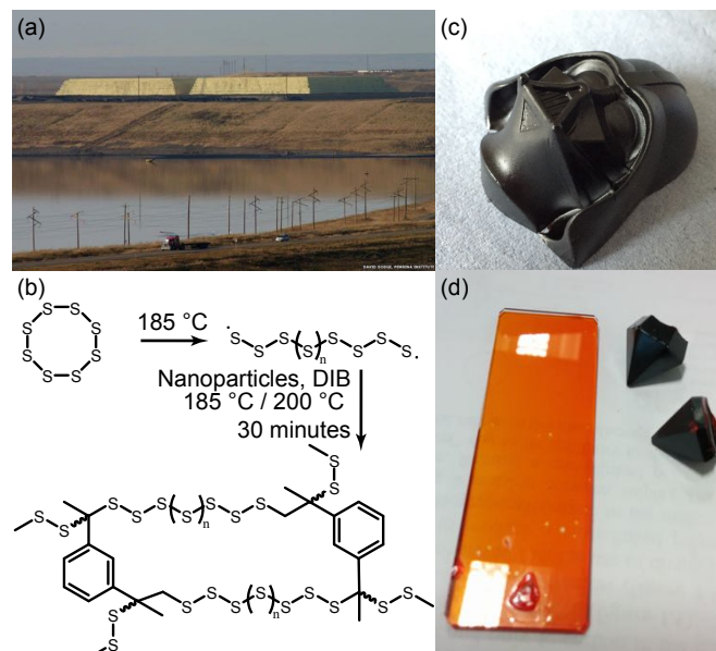
Fig. 1 (a) Sulphur wastes at Athabasca, Canada. Image used with permission: David Dodge, The Pembina Institute - www.pembina.org , (b) Scheme for formation of crosslinked polymer. (c) Moulded polymer containing Fe 3 O 4 nanoparticles, (d) Raw polymer (no nanoparticles) in film and moulded forms.
