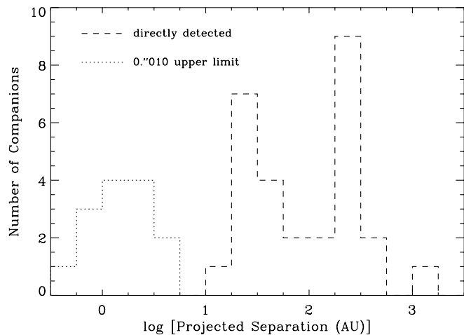
FIG. 3.—Distribution of projected separations for targets from Tables 3 and 4. The bin size is 0.25 in logarithmic AU, with identical bounds. The dashed line represents directly detected companions, while the dotted line represents upper limits of 0.010 for those binaries which remained unresolved.
