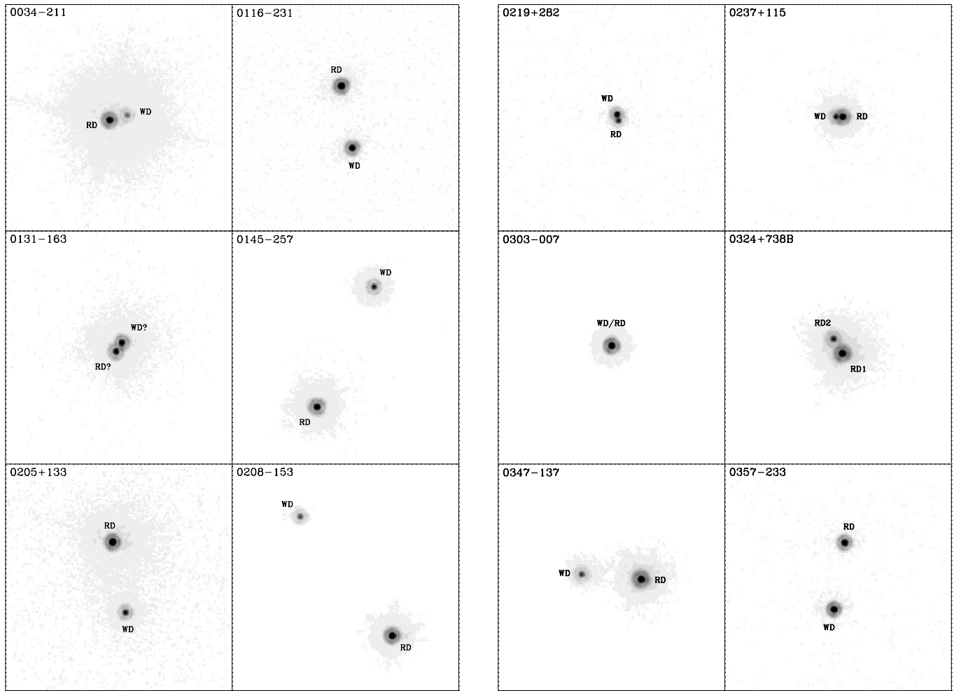
FIG. 1.—Multidrizzled images of the ACS HRC data taken in the F814W filter of all 28 totally or partially resolved multiple systems, plus an example of a single unresolved point source (0303–007). The images are 4'' \times 4'' ( 0''.025 pixels) with north up and east left.
