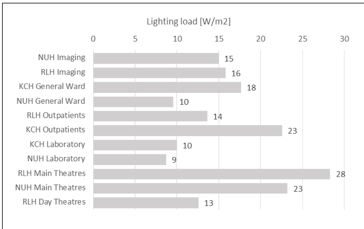
Figure 4: Departmental lighting loads
