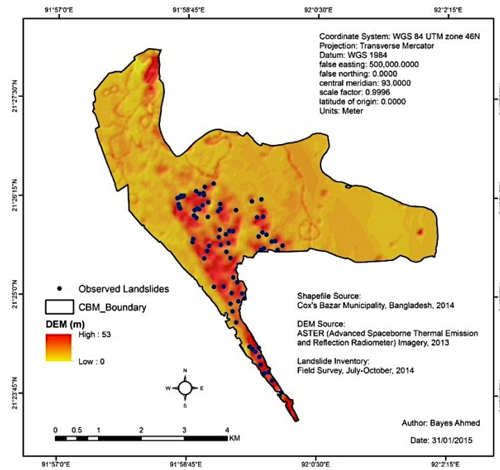
Figure 4. Landslide inventory map of CBM. Source: Ahmed, 2015a.
