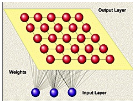
Figure 5. Example of the architecture of a SOM with an input layer (made up of three neurons) and an output layer (made up of 5 × 5 neurons). Source: Eastman, 2012.
