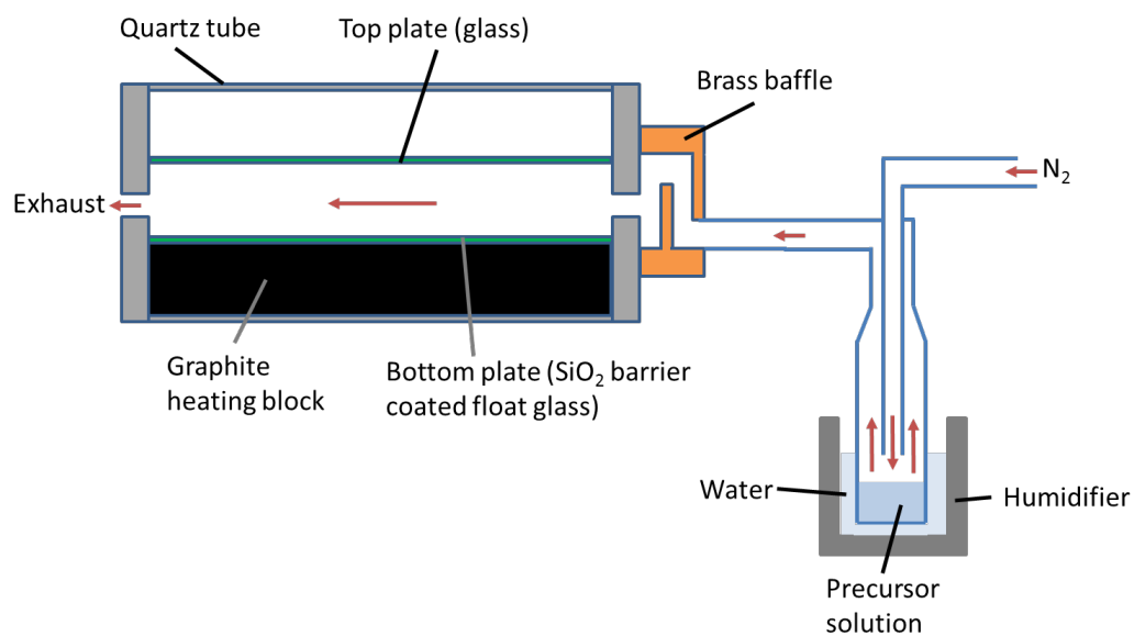
Figure 1 (SI): The Schematic diagram of the AACVD system. The aerosol of the precursor solution is created by plaining the bubbler into a humidifier that contains water. The aerosol is passed into the CVD chamber using a N 2 gas flow.
