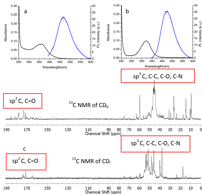
Fig. 3 UV-vis absorbance and photo luminescent emission spectra (excited at 360nm) of the carbon dots passivated with (a) branched PEI (CD b ) and (b) linear PEI (CD l ). (c) 13 C NMR spectrum of CD b and CD l .
