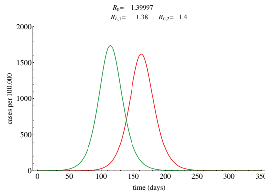
Figure 12. Epidemic curves of Canada (region 1, red, peak time: day 160) and Mexico (region 2, green, peak time: 117) when peak times were fitted to the real morbidity data of the first wave of the 2009 H1N1 outbreak and day 0 corresponds to December 31, 2008. Travel rates arise from [14], and historical peak times (day 117–123 in Mexico, day 155–162 in Canada) were derived from [21, 24, 39]. We set \mathcal{R}_{L,1} = 1.38 , \mathcal{R}_{L,2} = 1.4 , \tau = 0.25 , \gamma_1^{-1} = \gamma_2^{-1} = 15 , \beta^T = 20 , \mu_E^{-1} = 1.4 , \mu_I^{-1} = 2.7 , \mu_A^{-1} = 4.1 , p = 0.6 , \rho = 0.1 .
