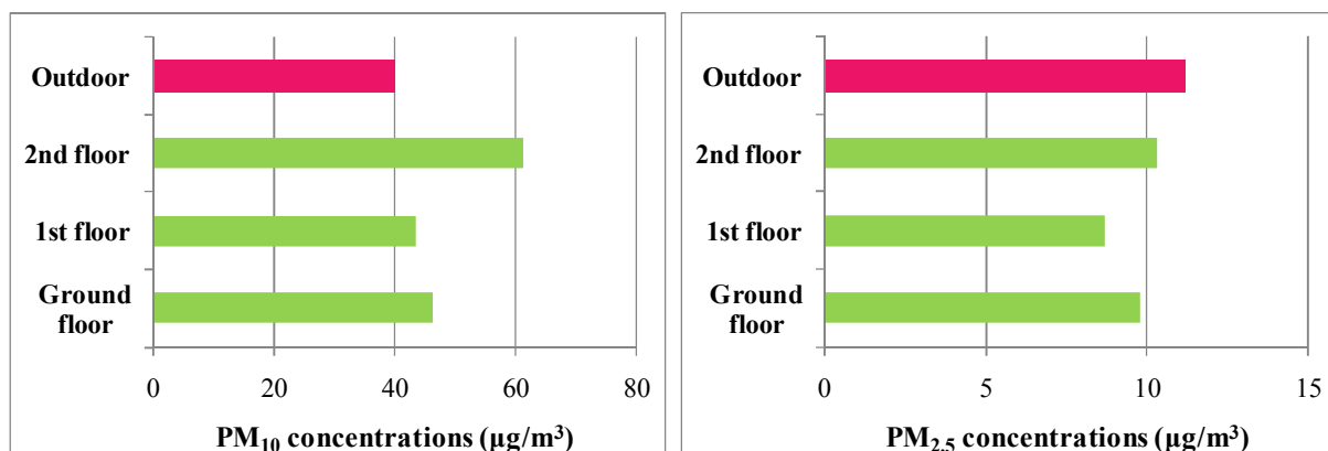
Figure 5: Averaged concentrations of PM10 (left) and PM2.5 (right) per floor in both of the schools
