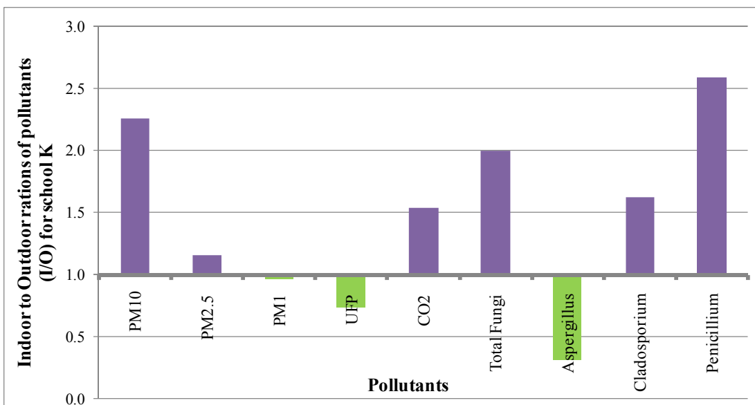
Figure 3: Indoor to outdoor (I/O) concentration ratios of pollutants in school K
