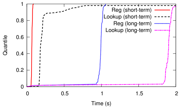
Fig. 2. Overall user-facing latency for the registration and lookup operations, excluding four network RTTs for registration and five for lookup.
