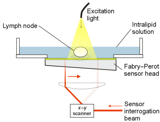
Fig. 1 Experimental setup for imaging lymph node samples.
