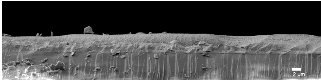
Figure 1: Side on SEM images of the AACVD film grown at (a) 500 °C and (b) 550 °C. The thickness of the film grown at 500 °C (a) is between 1-2 μm while the thickness of the 550 °C (b) ranges between 3 to 4 μm.
