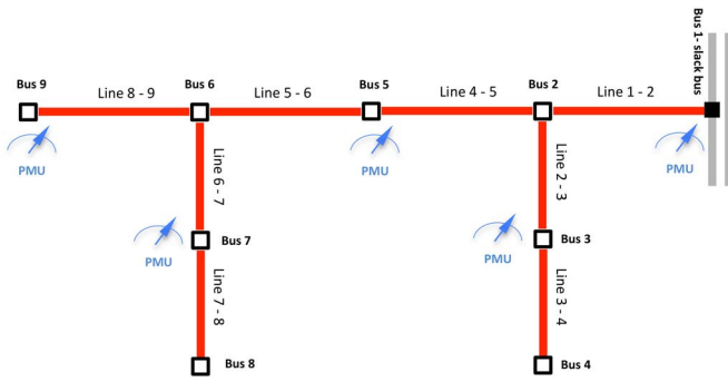
Fig. 4. Feeder used for proof-of-concept prototype experimentation.
