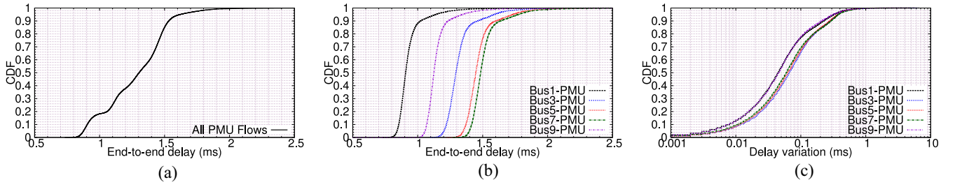
Fig. 7. End-to-end delay and delay variation of PMU flows in the prototype. (Color in online version.) (a) End-to-end delay across all PMU flows. (b) End-to-end delay per PMU flow. (c) Delay variation per PMU flow.
