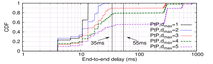
Fig. 11. End-to-end delay for the PtP approach (color in online version).
