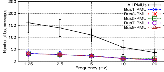
Fig. 8. Packet loss as a function of Hello message frequency (color in online version).
