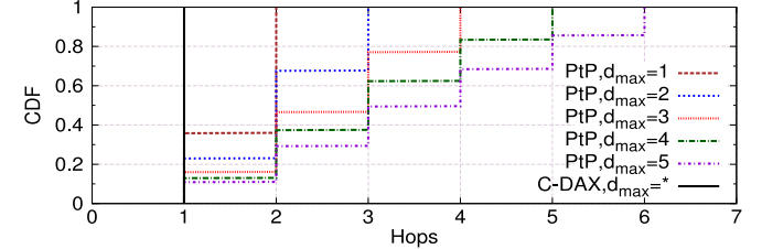
Fig. 12. PMU reconfiguration: distance traveled by control messages (color in online version).
