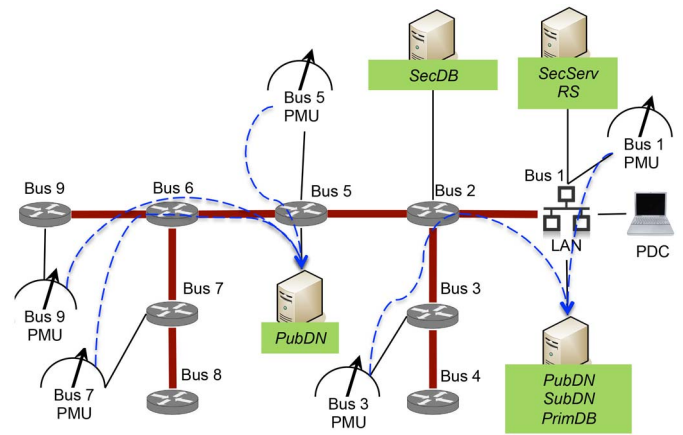
Fig. 5. C-DAX deployment on the feeder.
