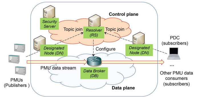
Fig. 2. C-DAX architecture.
