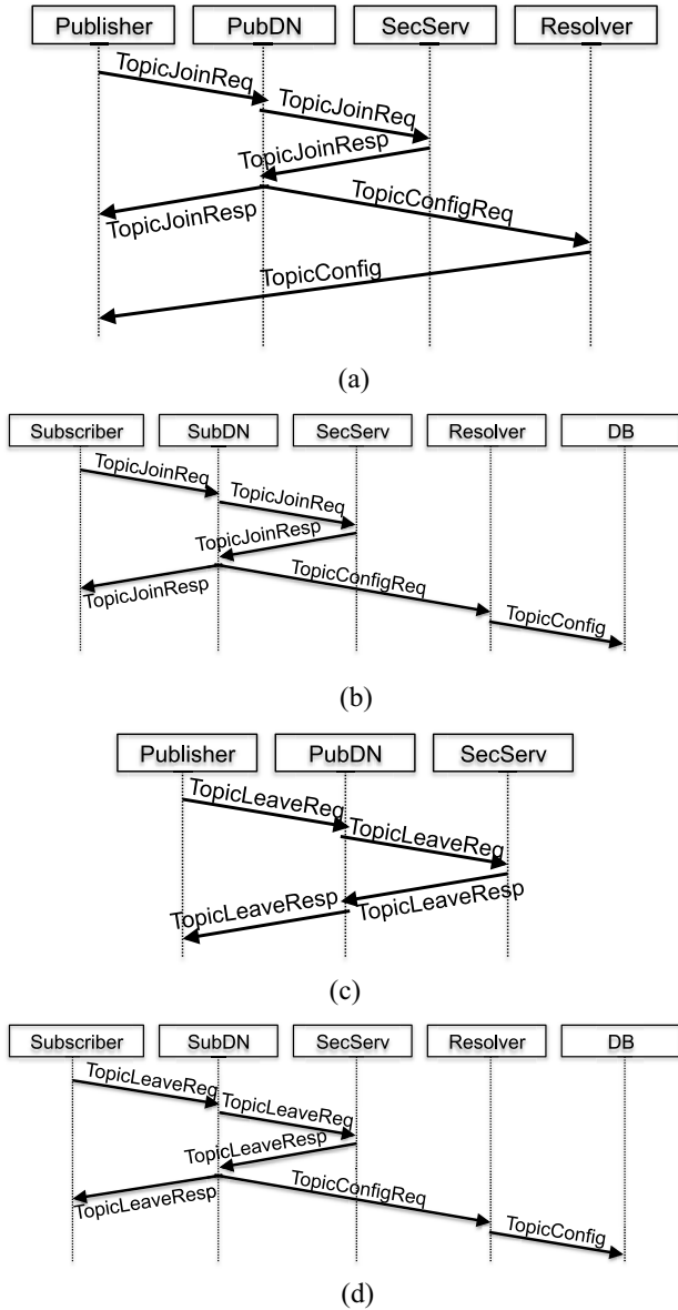
Fig. 3. Topic join/leave signaling sequences for publishers (e.g., PMUs) and subscribers (e.g., PDCs) who are decoupled spatiotemporally. (a) Publisher join. (b) Subscriber join. (c) Publisher leave. (d) Subscriber leave.
