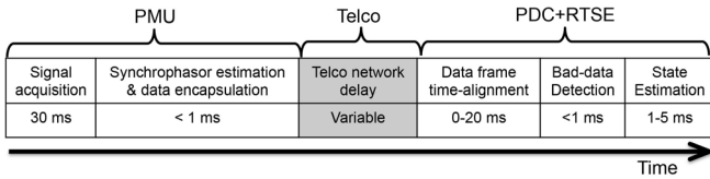
Fig. 1. Latency components of the entire RTSE process.
