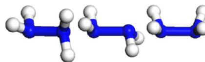
Figure 1. Representation of the N 2 H 4 conformations, from left to right: gauche, trans, and eclipsed.
