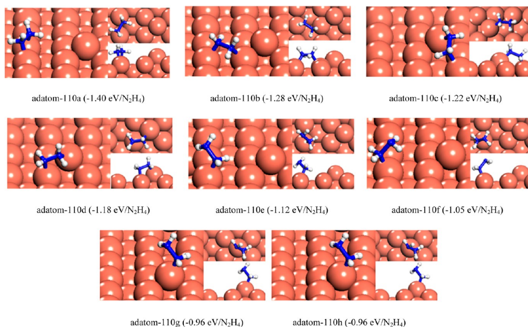
Figure 12. Lowest-energy configurations for adsorption of \text{N}_2\text{H}_4 on the adatom Cu (110) surface. (Adsorption energies are given in parentheses.)
