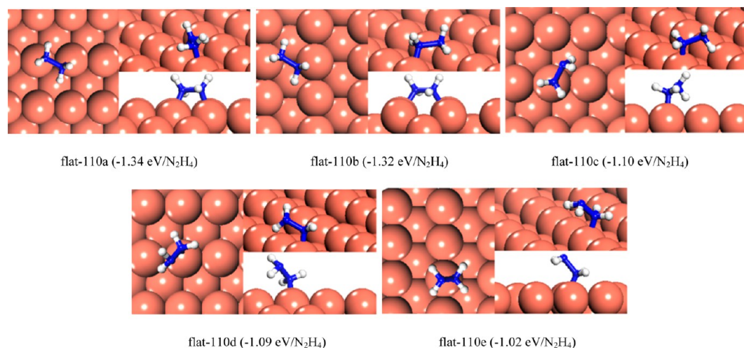
Figure 10. Lowest-energy configurations for adsorption of \text{N}_2\text{H}_4 on the perfect Cu(110) surface. (Adsorption energies are given in parentheses.)
