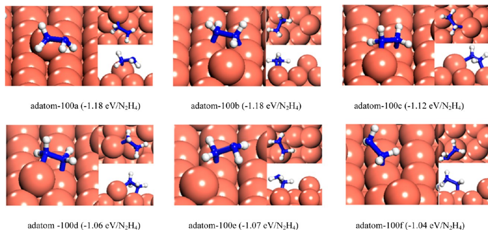
Figure 8. Surface geometry of the lowest-energy configurations for adsorption of \text{N}_2\text{H}_4 on the adatom Cu(100) surface. (Adsorption energies are given in parentheses.)
