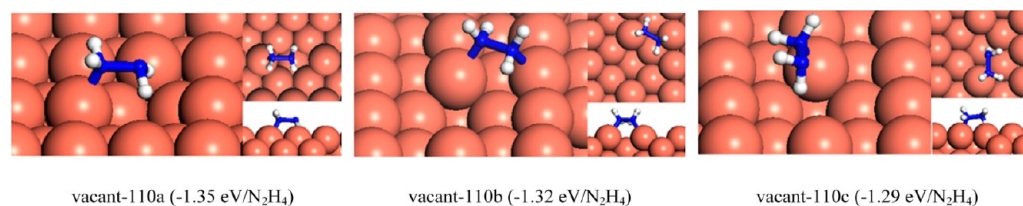
Figure 13. Lowest-energy configurations for adsorption of \text{N}_2\text{H}_4 on the Cu(110) vacancy surface. (Adsorption energies are given in parentheses.)
