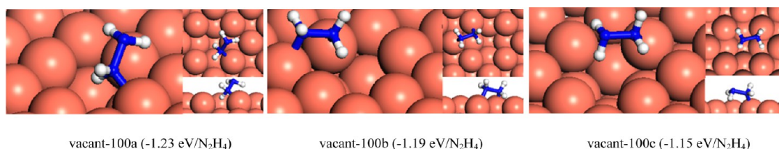
Figure 9. Lowest-energy configurations for adsorption of \text{N}_2\text{H}_4 on the Cu(100) vacancy surface. (Adsorption energies are given in parentheses.)
