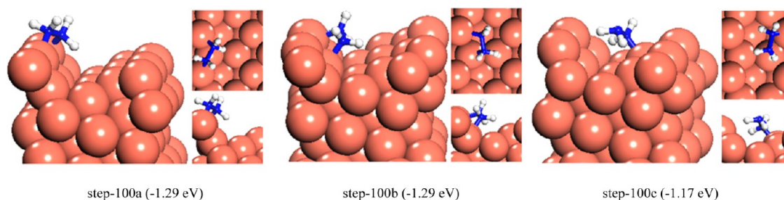
Figure 7. Lowest-energy configurations for adsorption of \text{N}_2\text{H}_4 on the stepped Cu(100) surface. (Adsorption energies are given in parentheses.)
