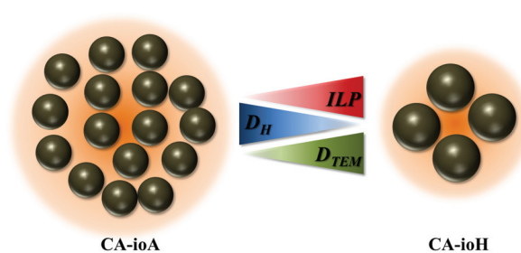
Scheme 1 Schematic of the observed correlation between the intrinsic loss parameter ILP, hydrodynamic diameter D_{\text{H}} , and core particle diameter D_{\text{TEM}} , for the citric acid coated multi-core iron oxide nanoparticles in this study. The increase in core size, together with the decrease in the hydrodynamic size, leads to a decrease of the number of cores per multi-core system ( N ), a decrease in the demagnetising interactions between those cores, and an increase in the ILP.
