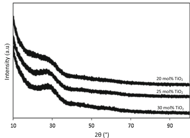
Fig. 3 XRD spectra of quaternary PCNT glasses
