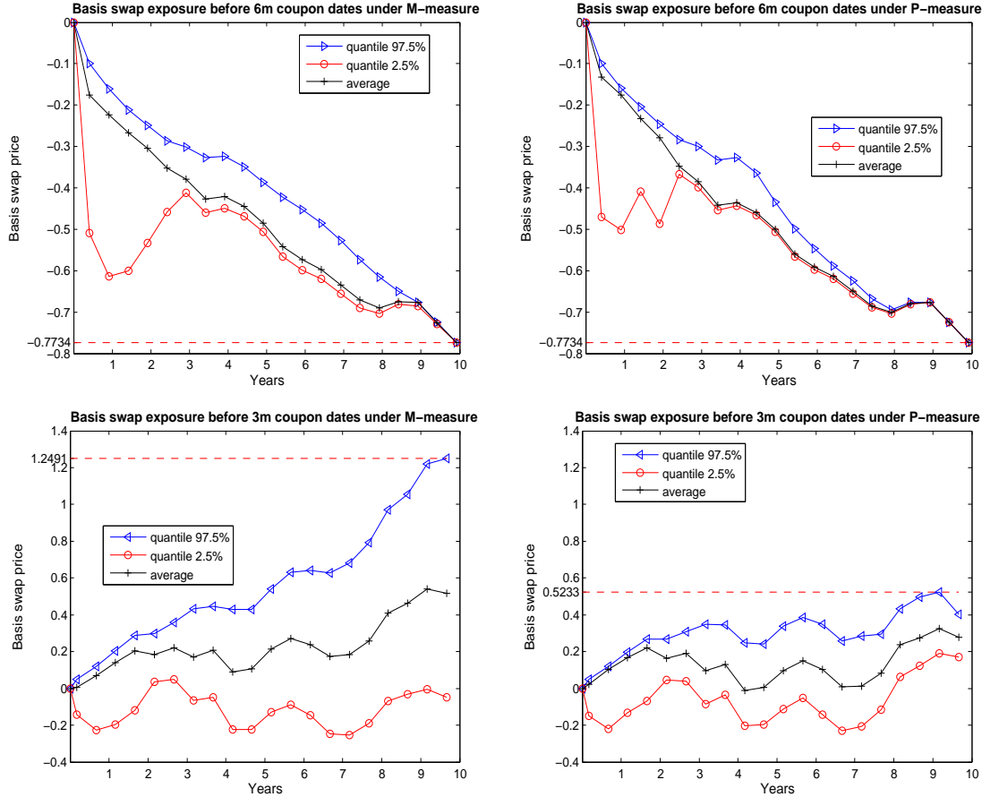
Figure 9: Exposures of a basis swap (price process with mean and quantiles) in the calibrated two-factor Gaussian model. ( Top ) Exposure of the basis swap at t = 5m, 11m, etc. ( Bottom ) Exposure of the basis swap price at t = 2m, 8m, 14m, etc. ( Left ) Exposure under the \mathbb{M} -measure. ( Right ) Exposure under the \mathbb{P} -measure with the prediction that the LIBOR rate L(10.75y; 10.75y, 11y) will be either 2% with probability p = 0.7 or 5% with probability 1 - p = 0.3 .
