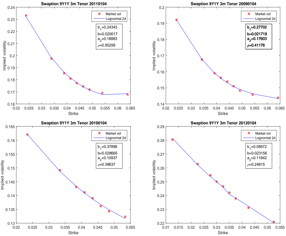
Figure 7: Lognormal two-factor calibration.
