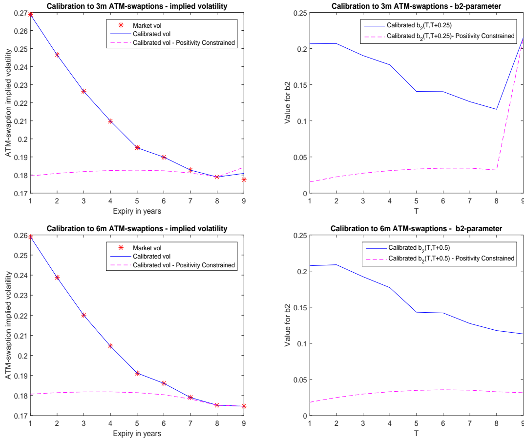
Figure 2: One-Factor Lognormal calibration. (Left) Fit to ATM swaption implied volatility term structures. (Right) Calibrated values of the b_2 parameters. (Top) \delta = 3m . (Bottom) \delta = 6m .
