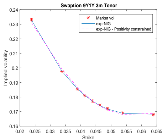
Figure 4: Exponential-NIG calibration
