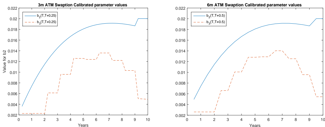
Figure 8: Two-factor lognormal calibration. (Left) Parameter values fitted to three-month ATM swaption implied volatility term structures. (Right) Parameter values fitted to six-month ATM swaption implied volatility term structures.
