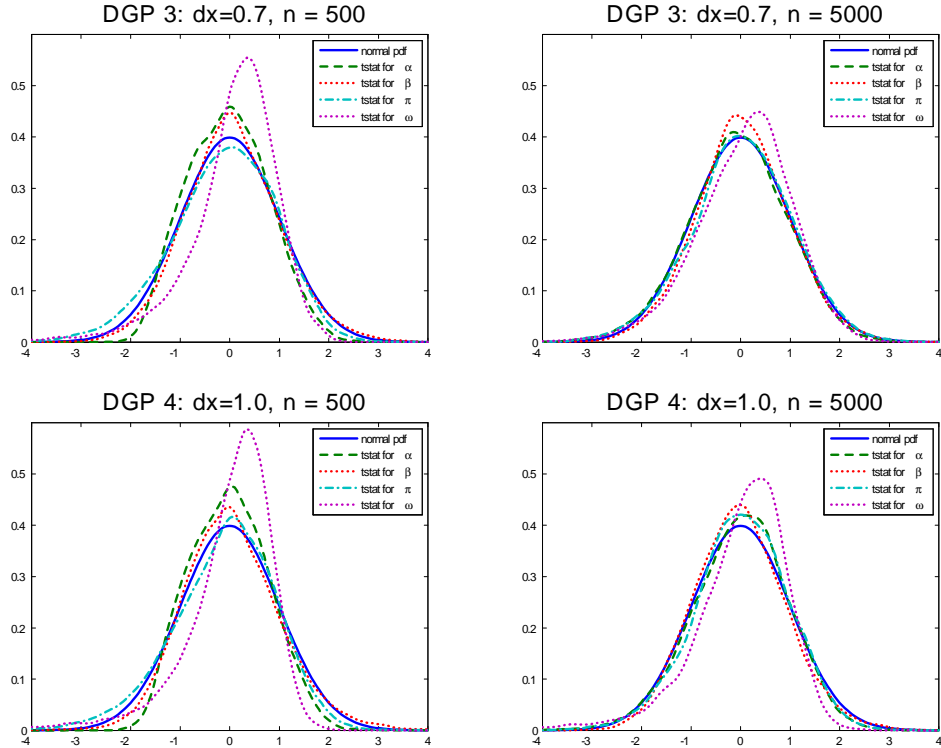
Figure 2. The simulated distributions of t -statistics for the nonstationary cases
