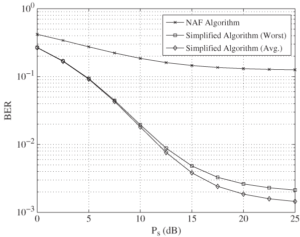
Fig. 4. Example 3: BER versus P_s . K = 3 , L = 3 , M = 2 , N_s = 2 , N_1 = 10 , N_2 = 6 , N_d = 10 , P_r = 20 dB.
