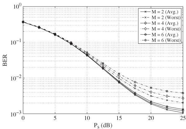
Fig. 5. Example 4: BER versus P_s . Varying number of receivers, K = 2 , L = 3 , N_s = 2 , N_1 = 6 , N_2 = 4 , N_d = 6 , P_r = 20 dB.
