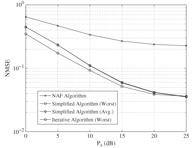
Fig. 2. Example 1: Normalized MSE versus P_s . K = 2, L = 3, M = 2, N_s = 2, N_1 = 8, N_2 = 4, N_d = 8, P_r = 20 dB.
