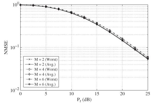
Fig. 3. Example 2: Normalized MSE versus P_r . Varying number of receivers, K = 2, L = 3, N_s = 2, N_1 = 6, N_2 = 4, N_d = 6, P_s = 20 dB.
