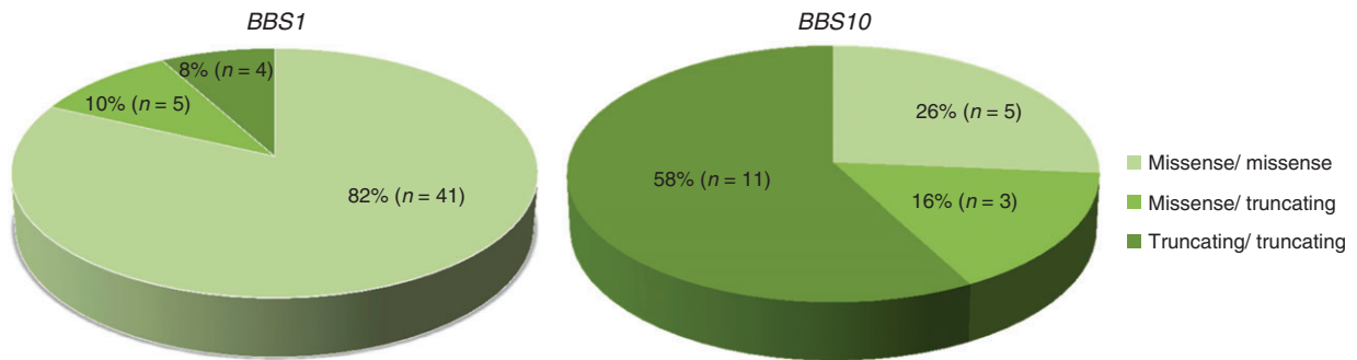
Fig. 1. Distribution of mutation type in patients with BBS1 and BBS10 included in the analysis.
