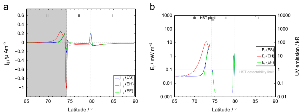
Fig. 6. (a) FAC densities in the high latitude ionospheric region for our transient expansion cases. The blue line represents case ES whilst the red and green lines indicate cases EH and EF, respectively. The conjugate magnetospheric regions (region III is shaded) are separated by dotted black lines and labelled. (b) The latitudinal variation of the precipitating electron flux (on the left axis) and the corresponding UV auroral emission (on the right axis) for the transient expansion cases. The colour codes and in plot labels are the same as in (a). The latitudinal size of an ACS-SBC HST pixel located near the main auroral emission is represented by the dark grey box. The solid grey line indicates the limit of detectability of the HST (Cowley et al., 2007).
