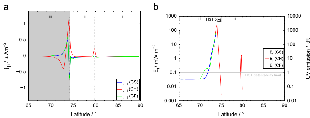
Fig. 3. (a) FAC densities in the high latitude ionospheric region for our transient compression cases. The blue line represents case CS whilst the red and green lines indicate cases CH and CF, respectively. The conjugate magnetospheric regions (region III is shaded) are separated by dotted black lines and labelled. (b) The latitudinal variation of the precipitating electron flux (on the left axis) and the corresponding UV auroral emission (on the right axis) for the transient compression cases. The colour codes and in plot labels are the same as in (a). The latitudinal size of an ACS-SBC HST pixel located near the main auroral emission is represented by the dark grey box. The solid grey line indicates the limit of detectability of the HST (Cowley et al., 2007).
