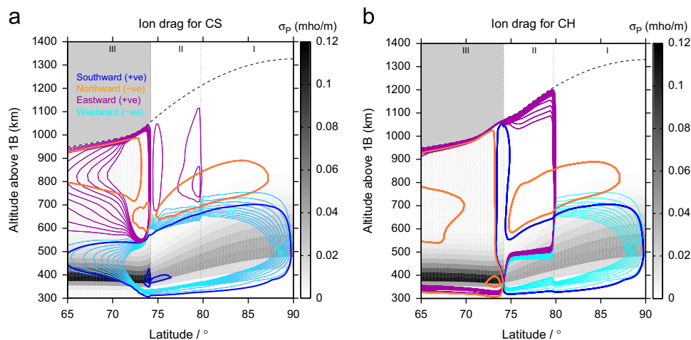
Fig. 9. (a) The variation of zonal and meridional ion drag momentum with altitude, latitude and Pedersen conductivity (colour bar) for case CS. The meridional contours (blue and orange) range from 1 to 500 \text{mm s}^{-2} with an interval of 50 \text{mm s}^{-2} and with blue being positive (southward) and orange being negative (northward). The zonal contours (purple and cyan) range from 1 to 10 \text{mm s}^{-2} with an interval of 1 \text{mm s}^{-2} and with purple being positive (eastwards) and cyan being negative (westwards). The magnetospheric regions are separated and labelled. (b) Variation of zonal and meridional ion drag momentum with altitude, latitude and Pedersen conductivity (colour bar) for case CH. All line styles and labels are as in (a).
