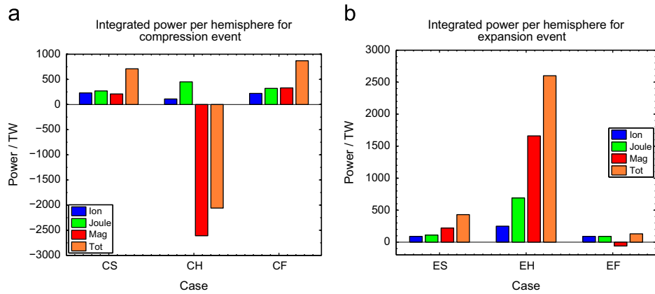
Fig. 10. (a) Integrated ionospheric powers per hemisphere for cases CS–CF are represented in this figure. Ion drag energy is represented by blue bars, Joule heating by green bars, magnetospheric power by red bars and total (sum of all above) is represented by orange bars. See text for further detail. (b) Integrated ionospheric powers per hemisphere for cases ES–EF are represented in this figure.
