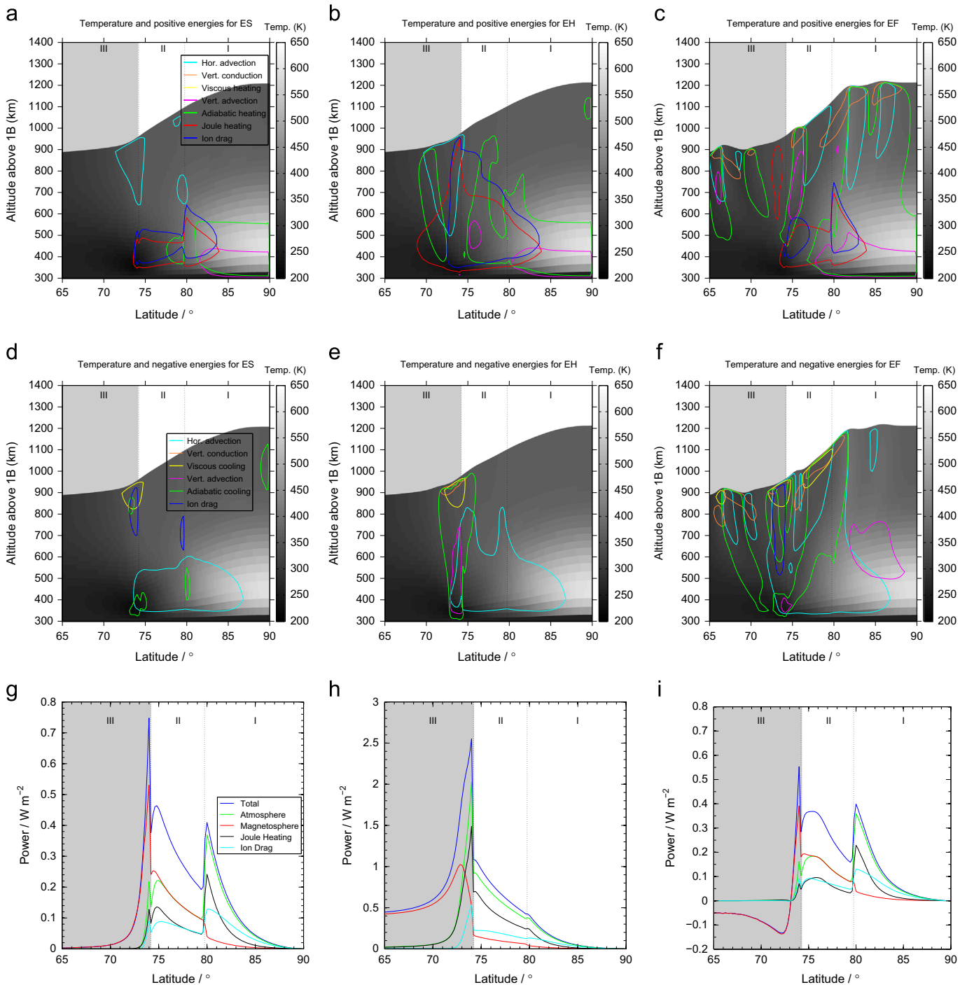
Fig. 8. (a)–(c) The variation of atmospheric heating terms with altitude, latitude and temperature (colour bar) for cases ES, EH and EF (left to right). The contours enclose regions where heating/kinetic energy rates exceed 20 \text{ W kg}^{-1} . Ion drag energy, Joule heating, vertical and horizontal advection of energy, adiabatic heating/cooling, viscous heating and heat conduction (vertical and turbulent) are represented by blue, red, yellow and magenta, green, cyan and orange lines. The magnetospheric regions are separated and labelled. (d)–(f) The variation of atmospheric cooling terms where the contours enclose regions where heating/kinetic energy are decreasing (cooling) with rates exceeding 20 \text{ W kg}^{-1} . All colours and labels are as in (a)–(c). (g)–(i) show how the power per unit area varies for our transient expansion cases. The blue line represents total power which is the sum of magnetospheric power (red line) and atmospheric power (green line); atmospheric power is the sum of both Joule heating (black solid line) and ion drag energy (cyan solid line). All other labels are as for (a)–(c).
