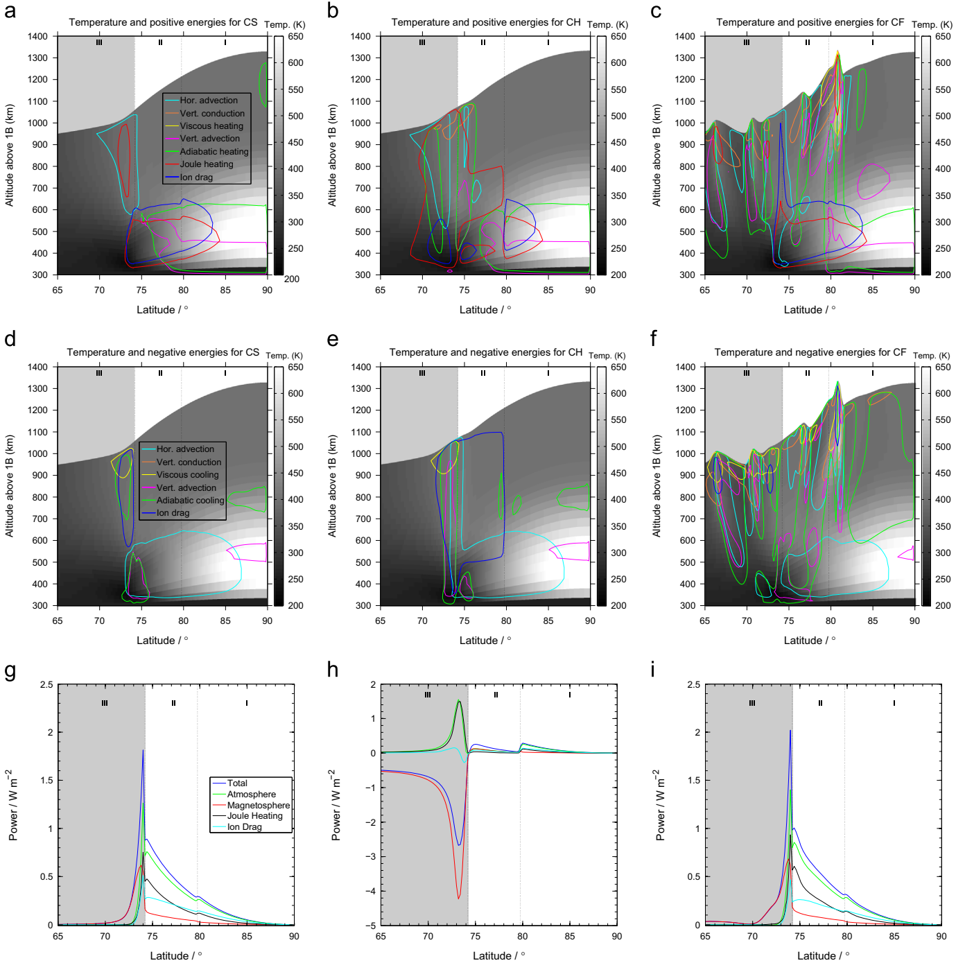
Fig. 5. (a)–(c) The variation of atmospheric heating terms with altitude, latitude and temperature (colour bar) for cases CS, CH and CF (left to right). The contours enclose regions where heating/kinetic energy rates exceed 20 \text{ W kg}^{-1} . Ion drag energy, Joule heating, vertical and horizontal advection of energy, adiabatic heating/cooling, viscous heating and heat conduction (vertical and turbulent) are represented by blue, red, yellow and magenta, green, cyan and orange lines. The magnetospheric regions are separated and labelled. (d)–(f) The variation of atmospheric cooling terms where the contours enclose regions where heating/kinetic energy are decreasing (cooling) with rates exceeding 20 \text{ W kg}^{-1} . All colours and labels are as in (a)–(c). (g)–(i) show how the power per unit area varies for our transient compression cases. The blue line represents total power which is the sum of magnetospheric power (red line) and atmospheric power (green line); atmospheric power is the sum of both Joule heating (black solid line) and ion drag energy (cyan solid line). Other labels are as for (a)–(c).
