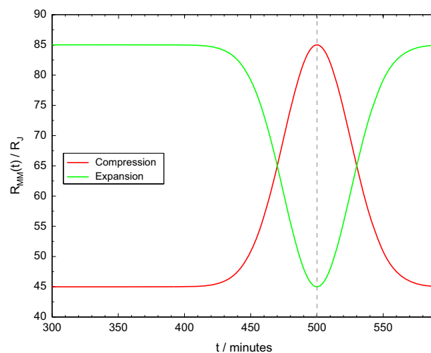
Fig. 1. The variation of magnetodisc radius R_{MM}(t) with time during a pulse in the solar wind. The red and green lines represent a compression and expansion respectively throughout the entire pulse. The grey dashed line indicates the point of maximum variation.
