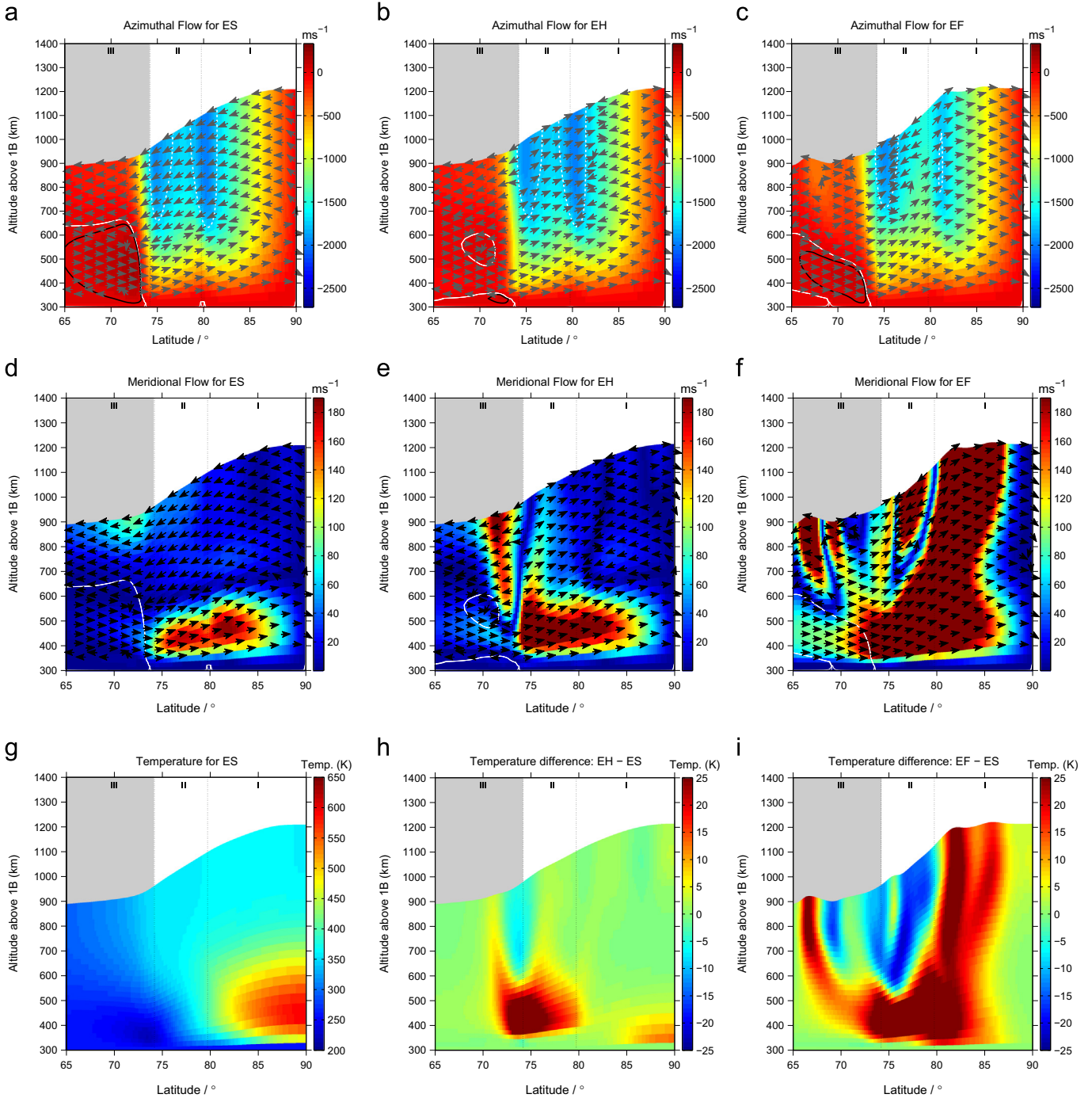
Fig. 7. (a)–(c) The variation of thermospheric azimuthal velocity (colour scale) in the corotating reference frame for cases ES–EF, respectively (left to right). Positive values (dark red) indicate super-corotation, whilst negative values (light red to blue) indicate sub-corotation. The arrows show the direction of meridional flow and the white line indicates the locus of rigid corotation. The solid black encloses regions of super-corotation ( > 25 \text{ m s}^{-1} ) and the dashed white line encloses regions that are sub-corotating at a rate < -1750 \text{ m s}^{-1} . The magnetospheric regions (region III is shaded) are separated by dotted black lines and labelled. (d)–(f) The meridional velocity in the thermosphere for cases ES–EF. The colour scale indicates the speed of flows. All other labels and are as for (a)–(c). (g) The thermospheric temperature distributions for case ES whilst (h)–(i) show the temperature difference between cases EH and EF and case ES. All labels are as in (a)–(c).
