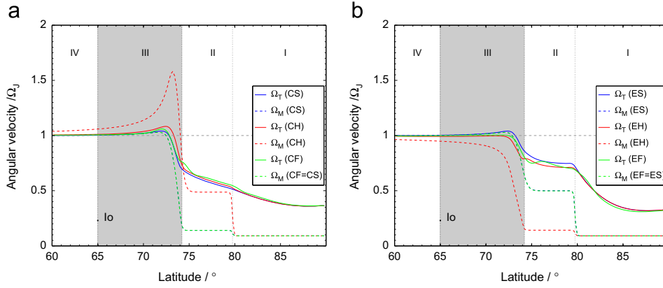
Fig. 2. (a) Thermospheric and plasma angular velocity profiles for the transient compression cases as a function of ionospheric latitude. Solid lines represent thermospheric profiles whilst dashed lines represent plasma profiles. The blue lines represent case CS (steady state before compression) whilst the red and green lines indicate cases CH (system at minimum disc radius) and CF (system just returned to initial disc radius) respectively. The magnetospheric regions (region III shaded) are labelled and separated by the black dotted lines. The magnetically mapped location of Io on the ionosphere is marked and labelled. (b) Thermosphere and plasma angular velocity profiles for the transient expansion cases as a function of ionospheric latitude. The line styles are the same as (a) but the cases are now ES, EH and EF respectively, where ‘E’ denotes expansion, and the ‘S’, ‘H’ and ‘F’ symbols represent the same phases of the event as for (a).
