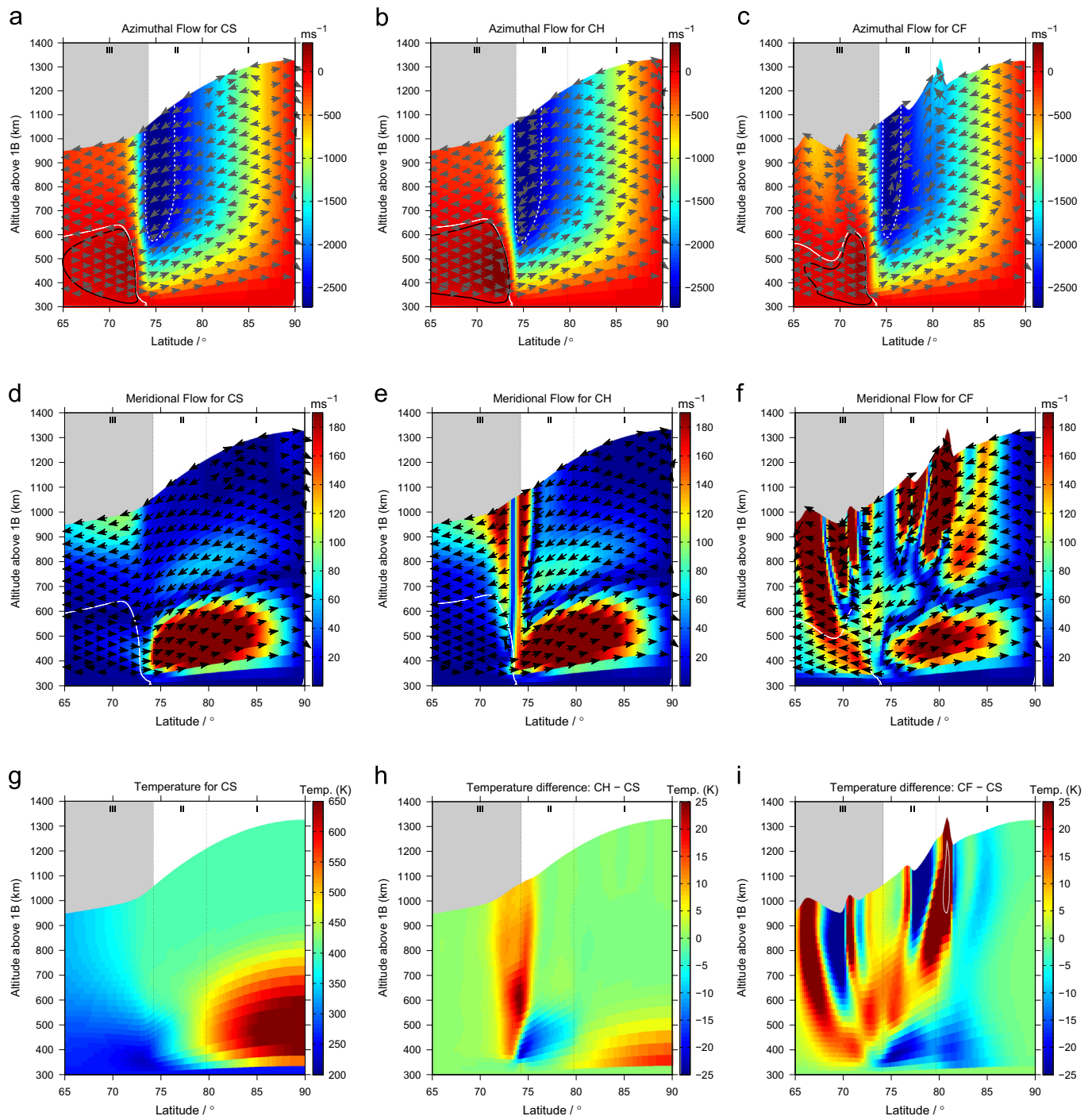
Fig. 4. (a)–(c) The variation of thermospheric azimuthal velocity (colour scale) in the corotating reference frame for cases CS–CF respectively (left to right). Positive values (dark red) indicate super-corotation, whilst negative values (light red to blue) indicate sub-corotation. The arrows show the direction of meridional flow and the solid white line indicates the locus of rigid corotation. The solid black encloses regions of super-corotation ( > 25 \text{ m s}^{-1} ) and the dashed white line encloses regions that are sub-corotating at a rate < -2500 \text{ m s}^{-1} . The magnetospheric regions (region III is shaded) are separated by dotted black lines and labelled. (d)–(f) The meridional velocity in the thermosphere for cases CS–CF. The colour scale indicates the speed of flows. All other labels and are as for (a)–(c). (g) The thermospheric temperature distributions for case CS whilst (h)–(i) show the temperature difference of cases CH and CF with case CS. The white contour encloses temperature differences > 100 \text{ K} . All labels are as in (a)–(c).
