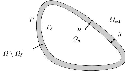
FIG. 1. The scattering layered object
