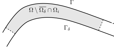
FIG. 2. Local covering of the layer
