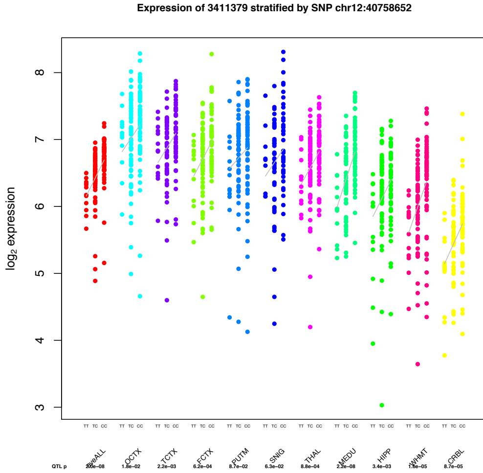
Figure S3: Expression genotype correlation in n = 134 brain samples for exon 33 of LRRK2 and SNP rs3761863 (M2397T, Crohn disease associated). All ten brain regions are shown.
