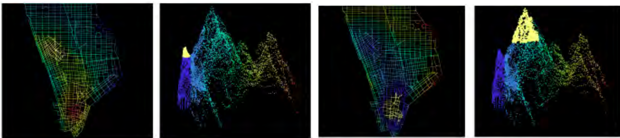
Figure 16: Peaks and patches in Manhattan
