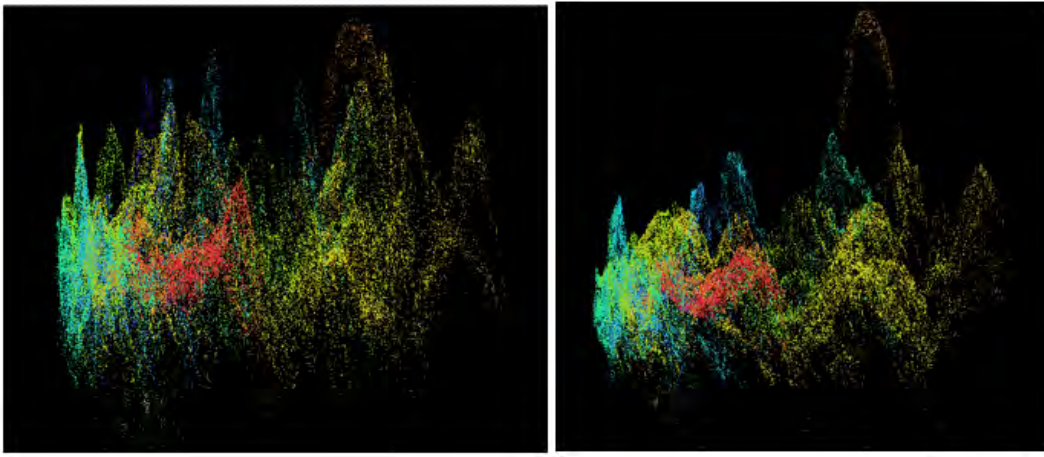
Figure 19: 'Mountain scattergrams for the areas of Istanbul at 500 and 1500 metres'
