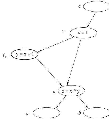
Fig. 4. Simple Example of a vertex (highlighted in bold) that need not be considered as a potential linchpin.
