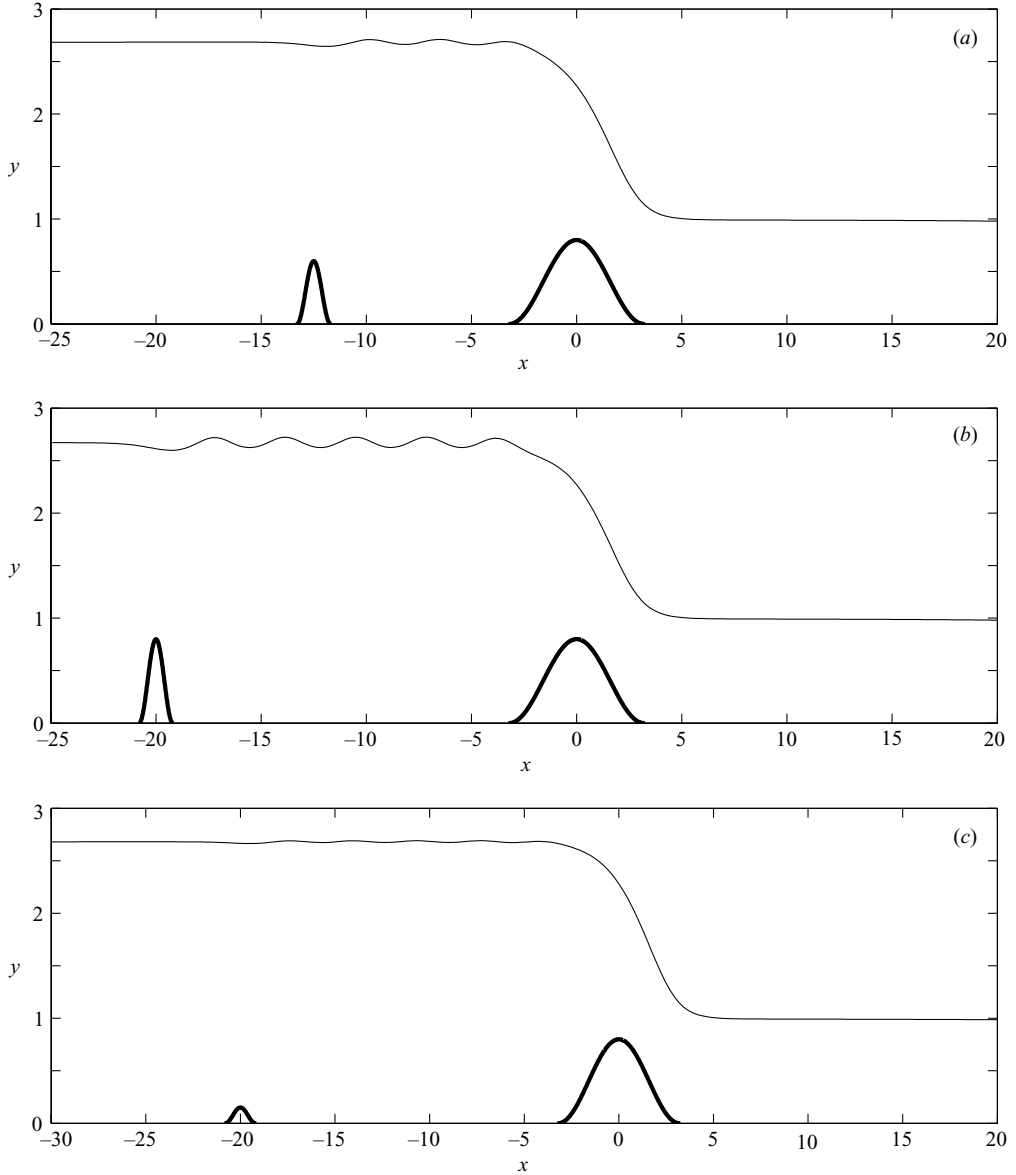
FIGURE 5. Computed hydraulic fall past two submerged obstacles in the shape of a cosine. Waves are trapped between the obstacles. The obstacles are characterized by A_2 = 0.4 , L_1 = 0.8 , L_2 = 3.2 , and (a) A_1 = 0.3 , l = 12.5 ; (b) A_1 = 0.4 , l = 20 ; (c) A_1 = 0.075 , l = 20 . The Froude number is found as part of the solution: (a) F = 1.976 , (b) F = 1.971 , (c) F = 1.976 .
