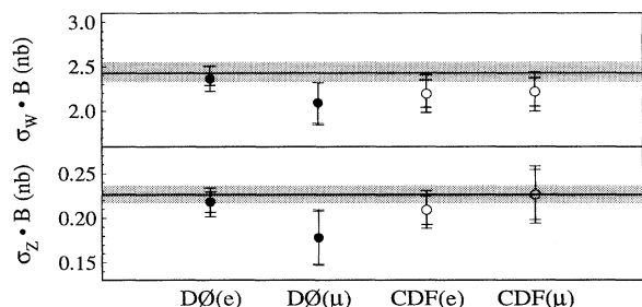
FIG. 2. \sigma B for inclusive W and Z boson production. The inner error bar is the combined statistical and systematic uncertainty and the outer error bar includes the luminosity uncertainty. The solid line and shaded band are the theoretical prediction described in the text.
