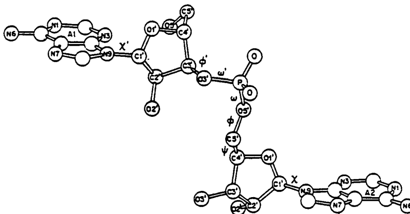
Figure 1. A single molecule of ApA. The conformational nomenclature for the torsion angles is shown.
